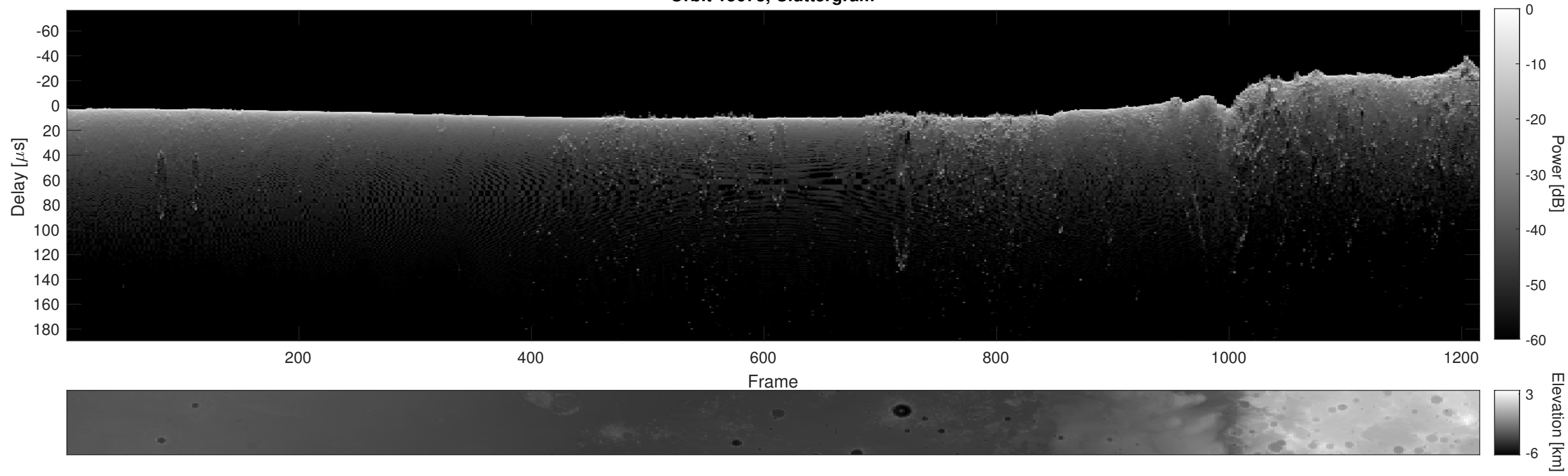
Orbit 15673, Cluttergram
