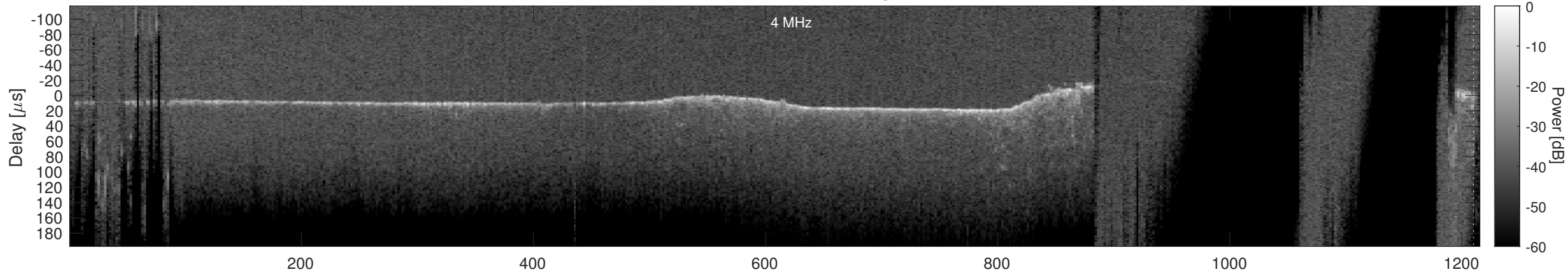
Orbit 15674, Cluttergram
