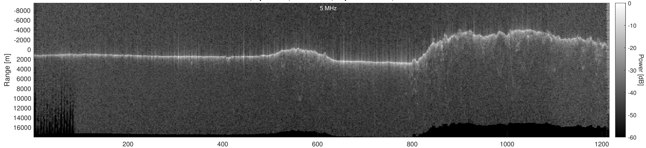
Orbit 15674, Optimized, No Window, Depth-Corrected, Channel 2
