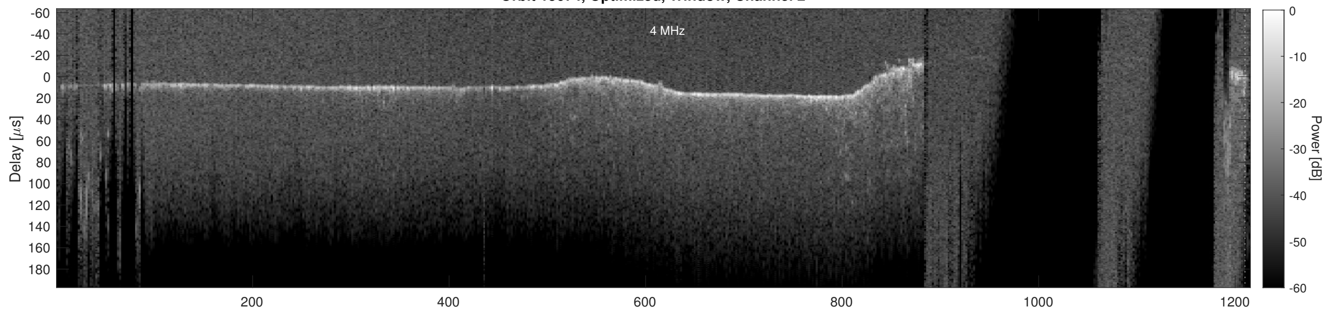
Orbit 15674, Cluttergram
