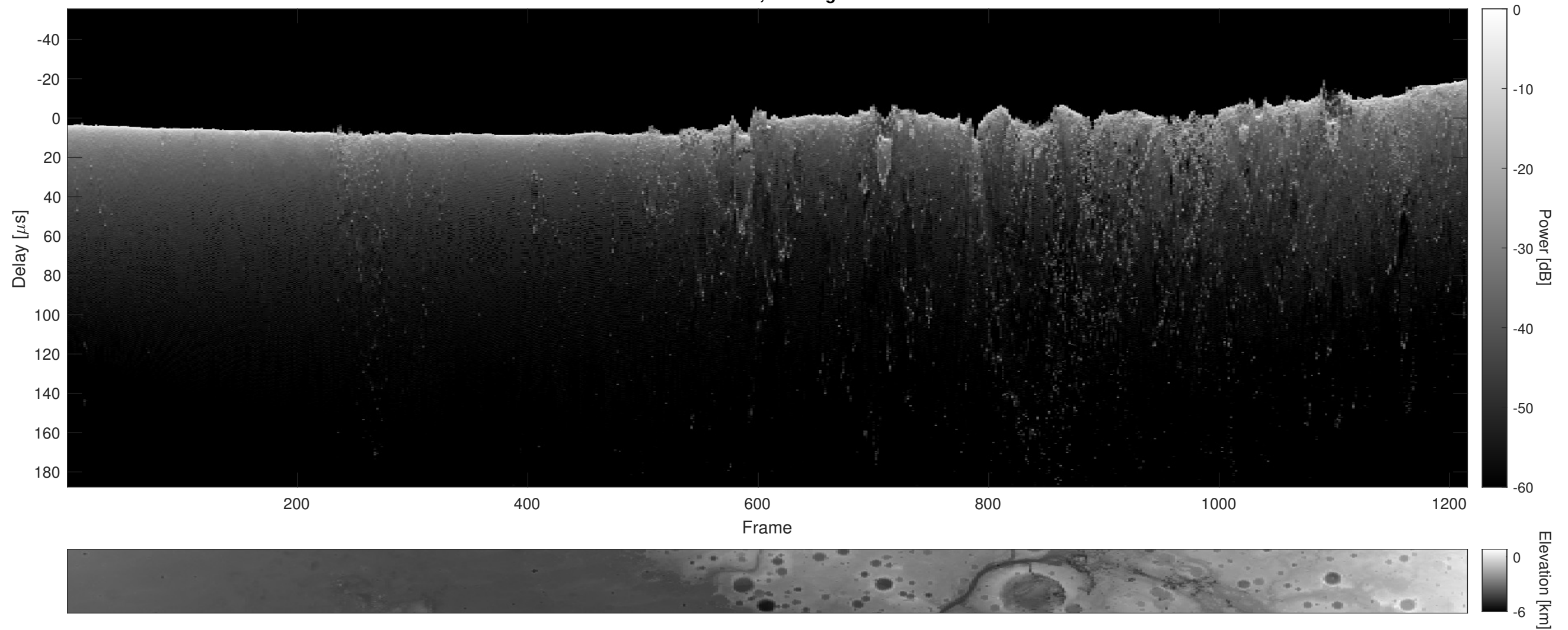
Orbit 15675, Cluttergram
