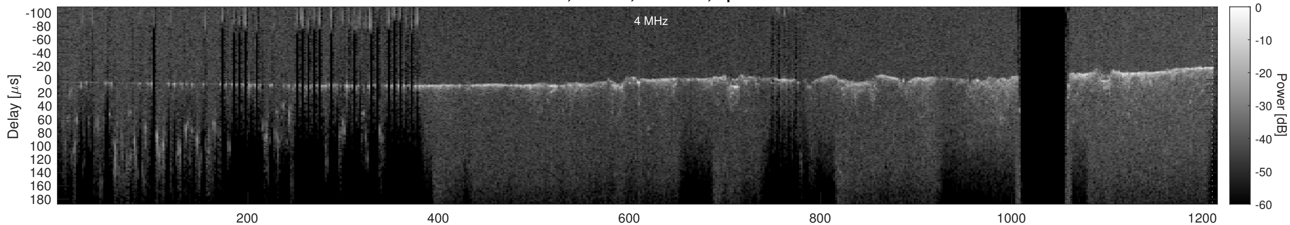
Orbit 15675, Cluttergram
