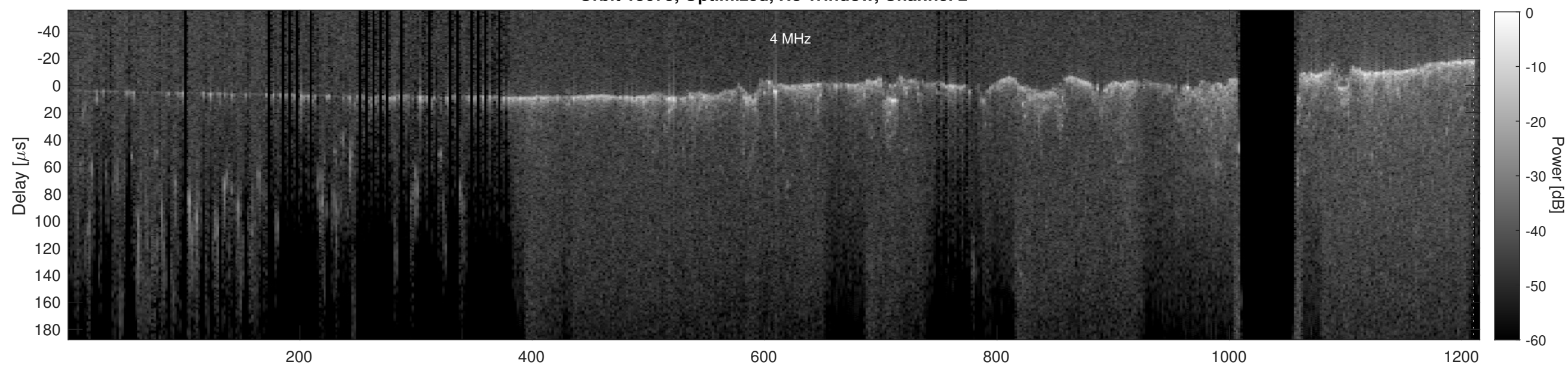
Orbit 15675, Cluttergram
