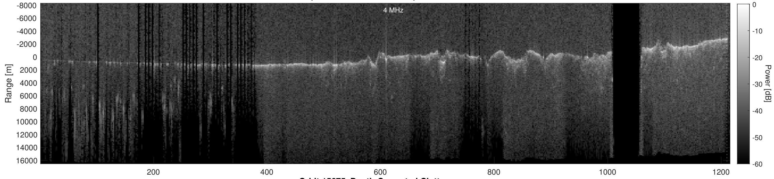
Orbit 15675, Depth-Corrected Cluttergram
