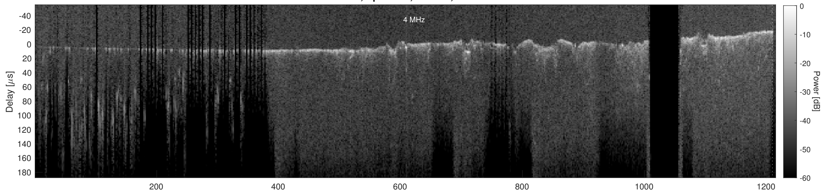
Orbit 15675, Cluttergram
