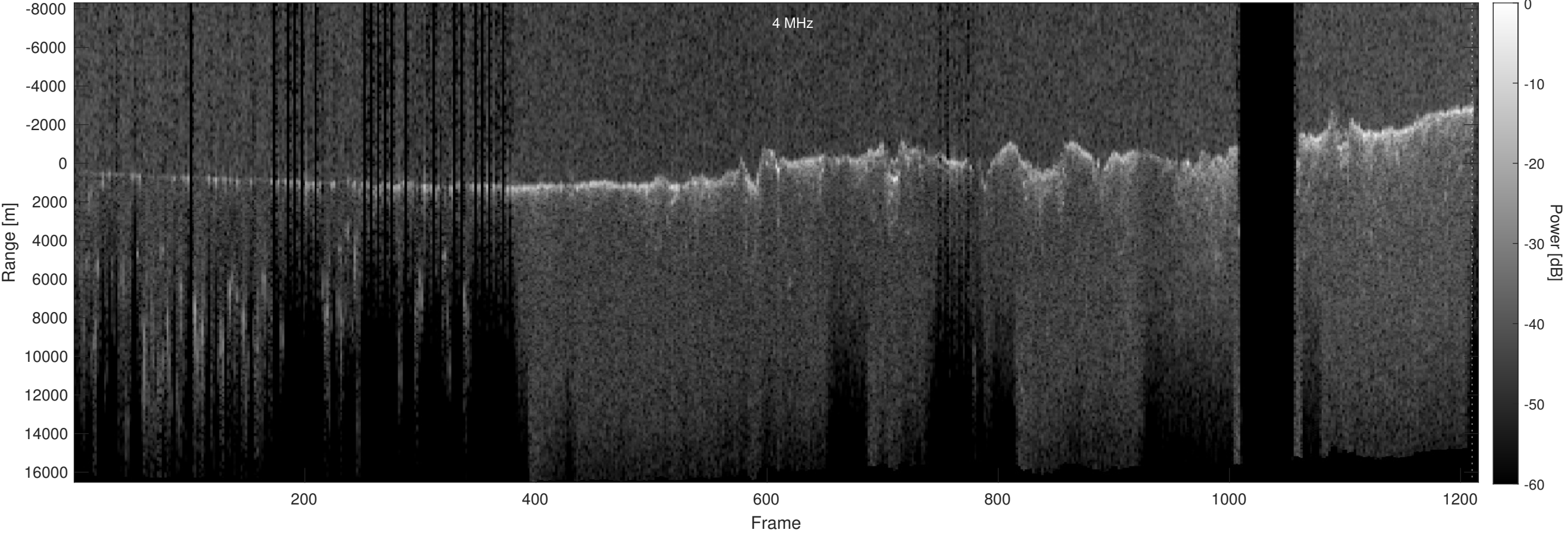
Orbit 15675, Optimized, Window, Depth-Corrected, Channel 2
