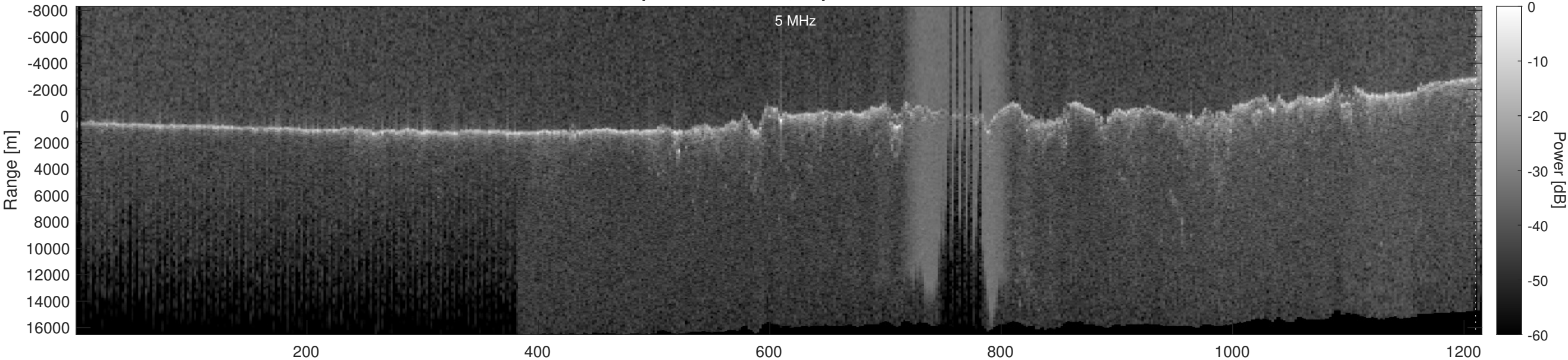
Orbit 15675, Optimized, Window, Depth-Corrected, Channel 2
