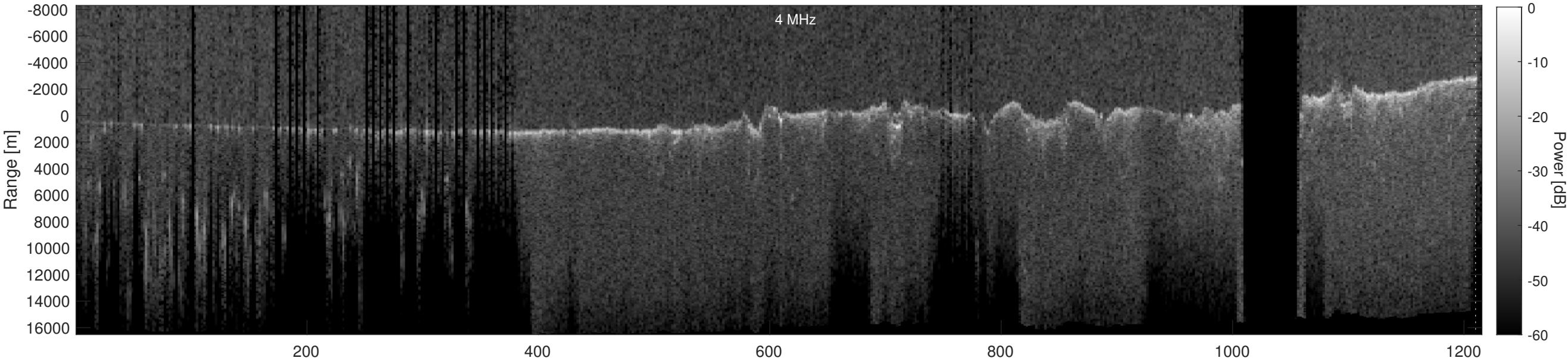
Orbit 15675, Depth-Corrected Cluttergram
