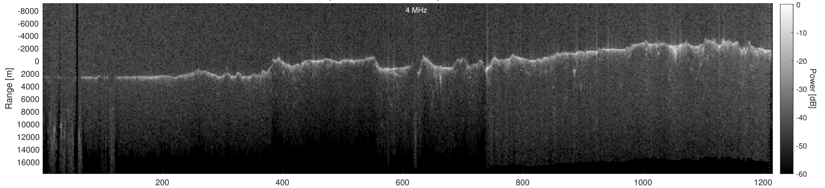
Orbit 15678, Depth-Corrected Cluttergram
