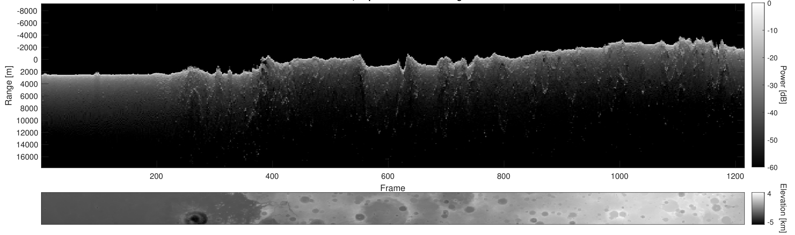
Orbit 15678, Depth-Corrected Cluttergram
