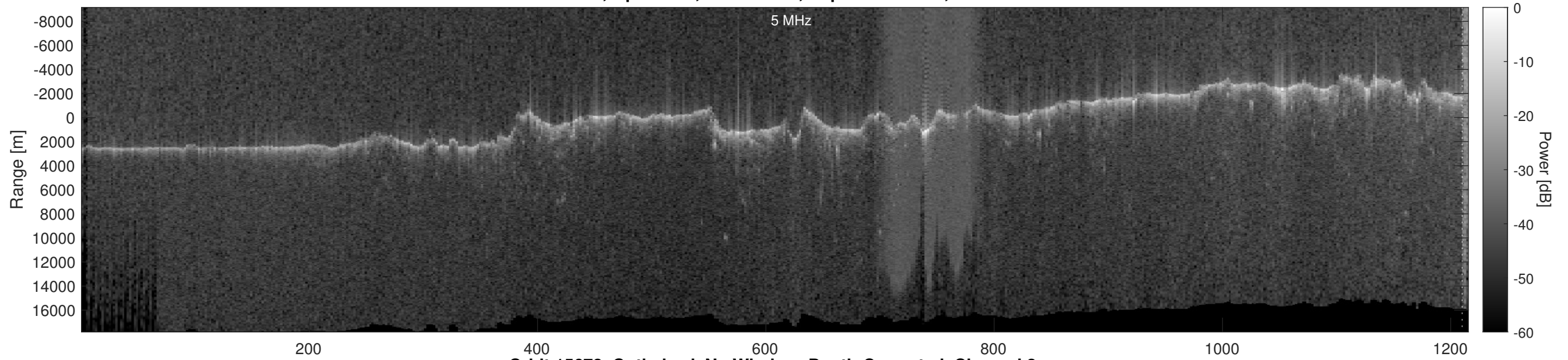
Orbit 15678, Optimized, No Window, Depth-Corrected, Channel 2
