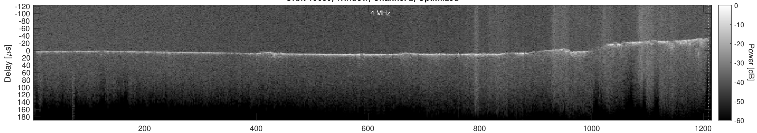
Orbit 15680, Cluttergram
