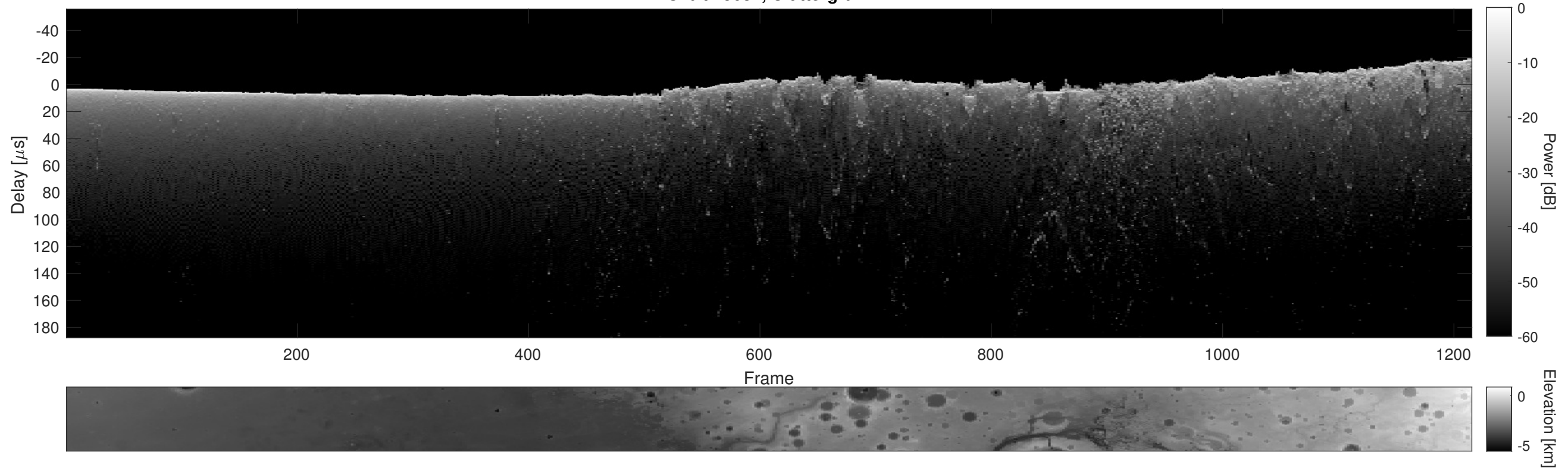
Orbit 15682, Cluttergram
