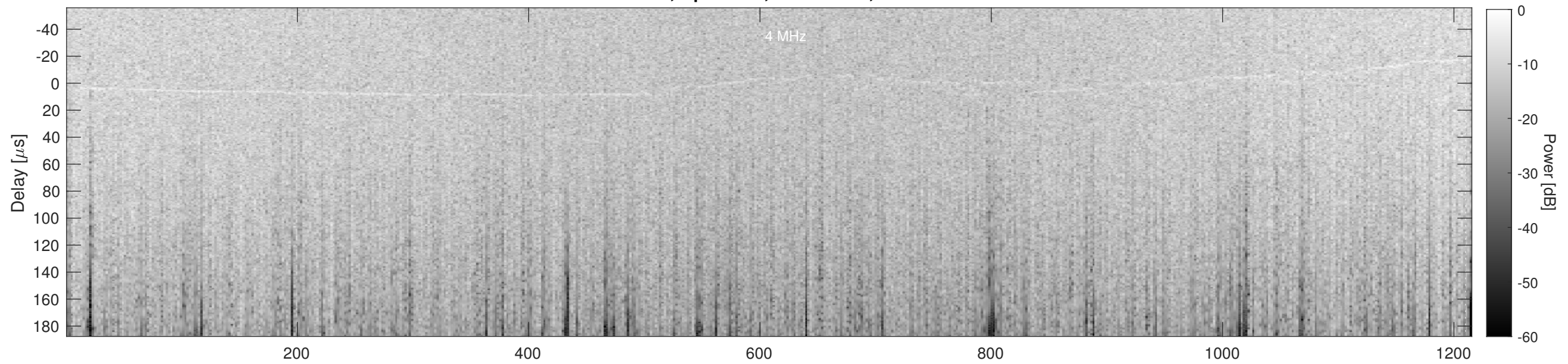
Orbit 15682, Cluttergram
