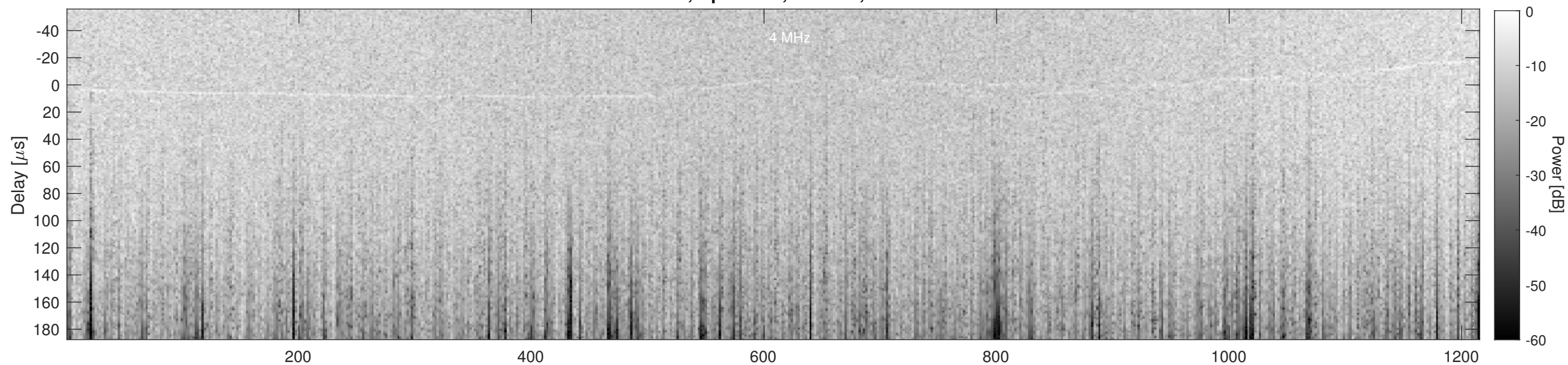
Orbit 15682, Cluttergram
