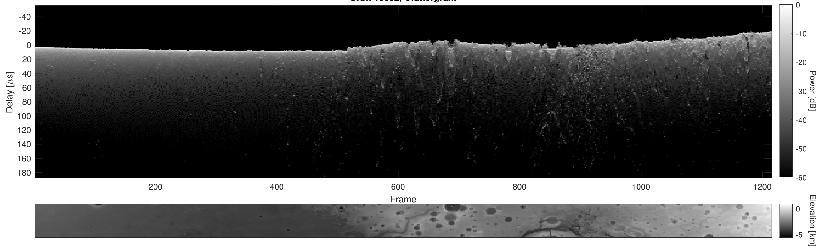
Orbit 15682, Cluttergram
