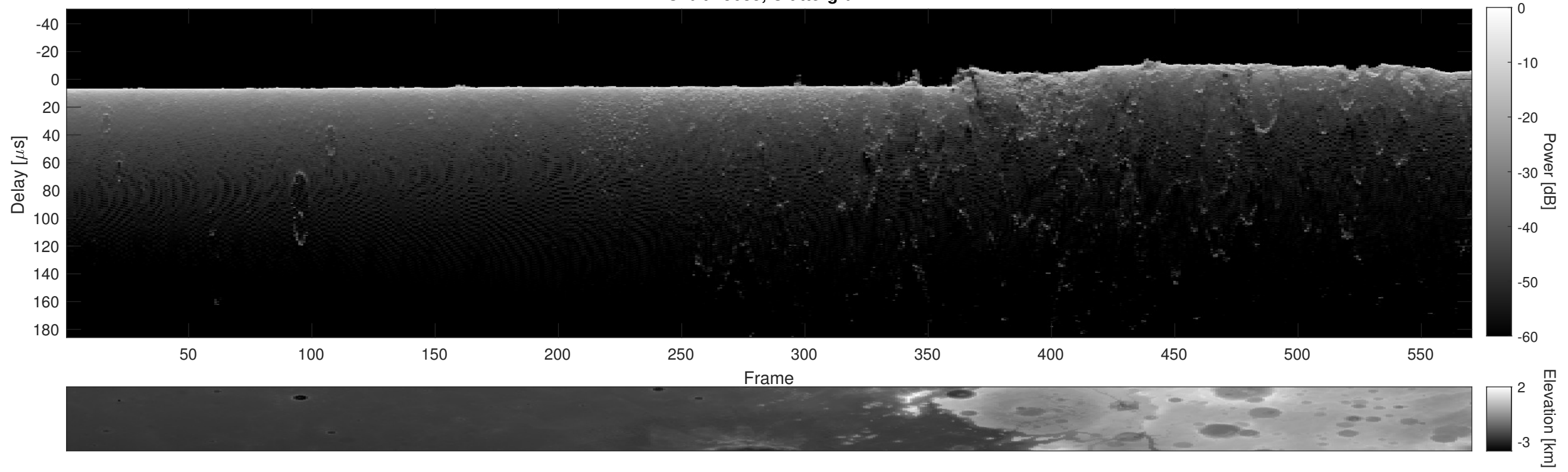
Orbit 15685, Cluttergram
