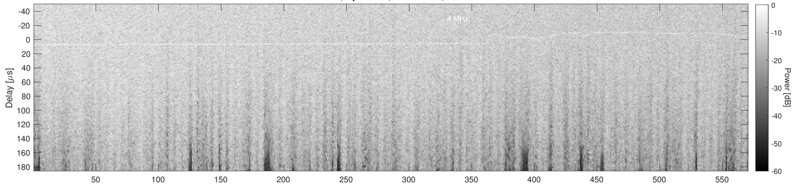
Orbit 15685, Cluttergram
