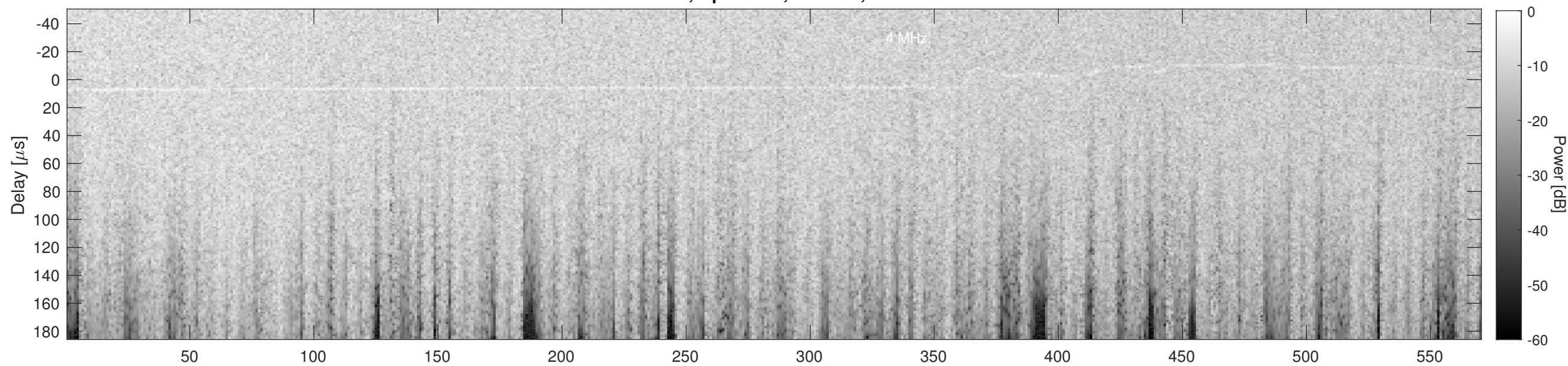
Orbit 15685, Cluttergram
