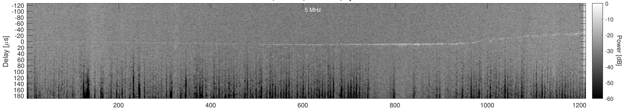
Orbit 15687, Cluttergram
