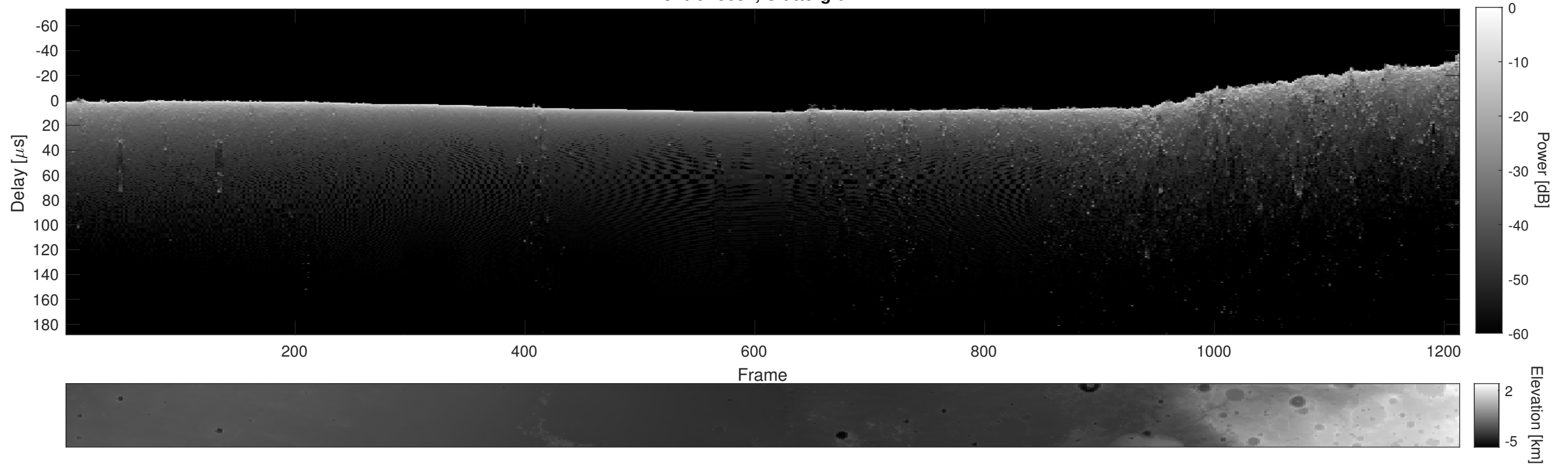
Orbit 15687, Cluttergram
