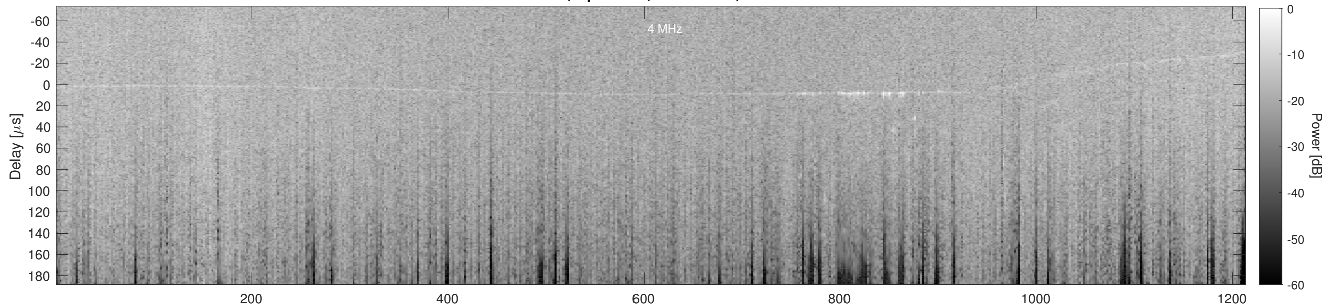
Orbit 15687, Cluttergram
