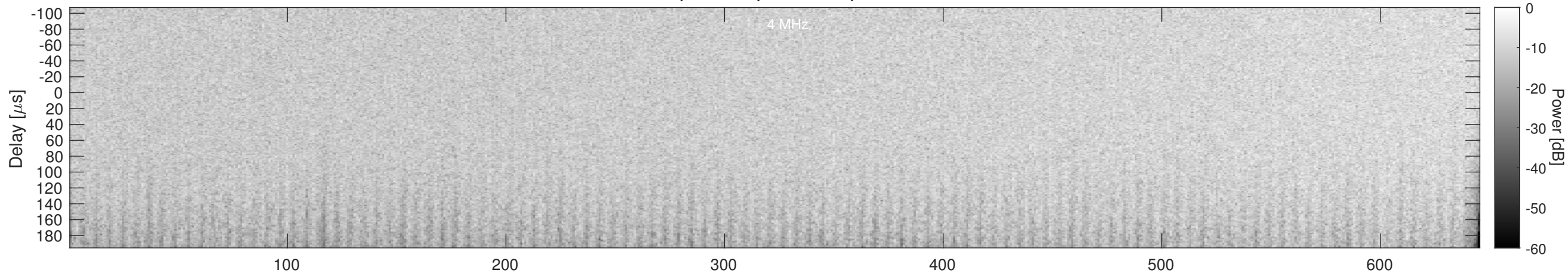
Orbit 15688, Window, Channel 2, Chapman
