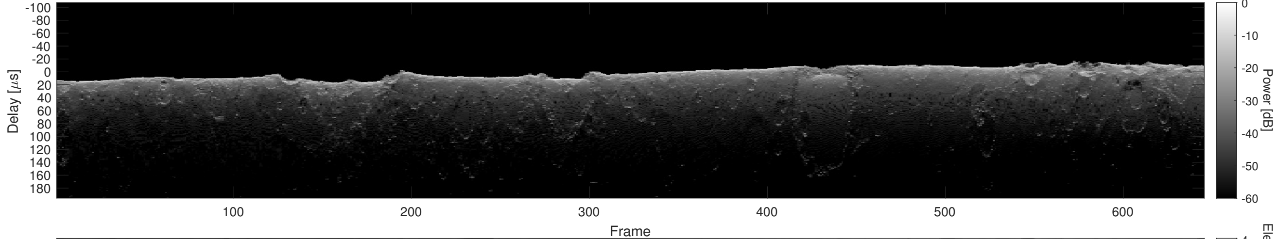
Orbit 15688, Cluttergram
