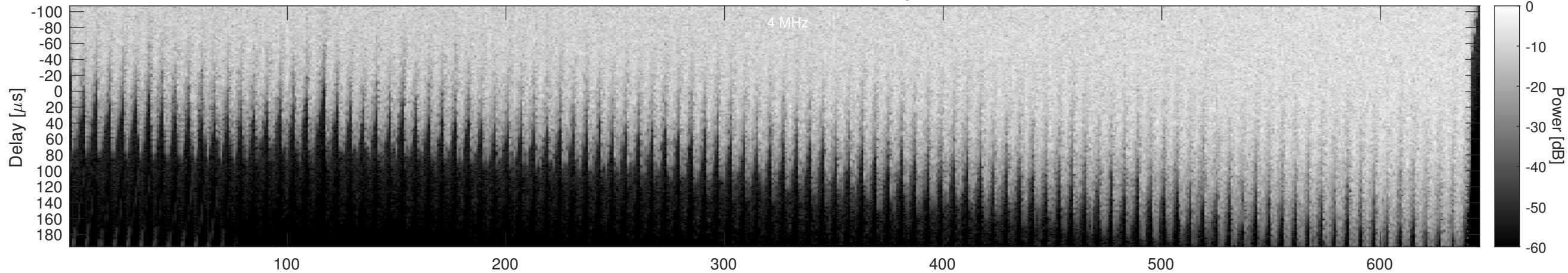
Orbit 15688, Window, Channel 2, Optimized
