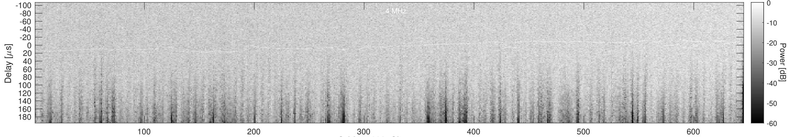
Orbit 15688, Cluttergram
