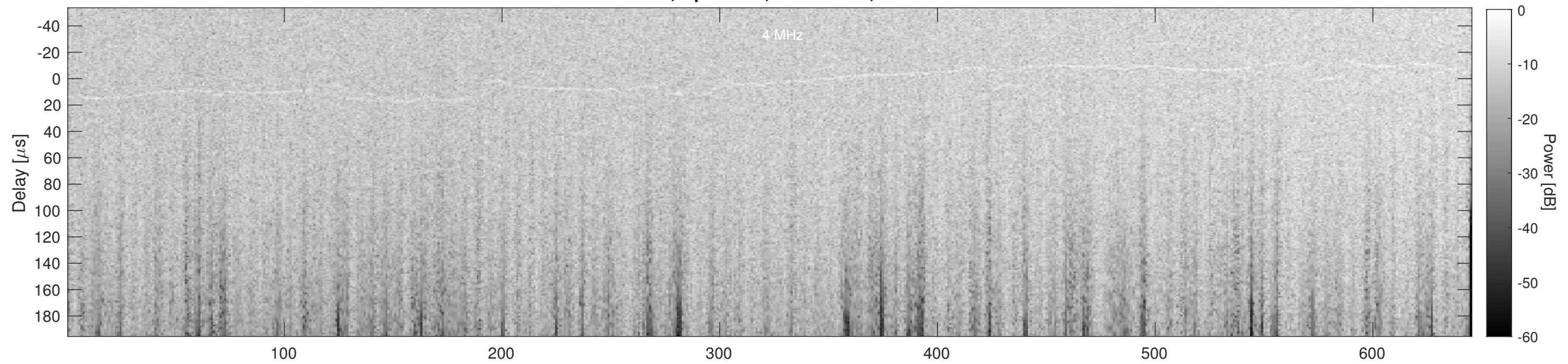
Orbit 15688, Cluttergram
