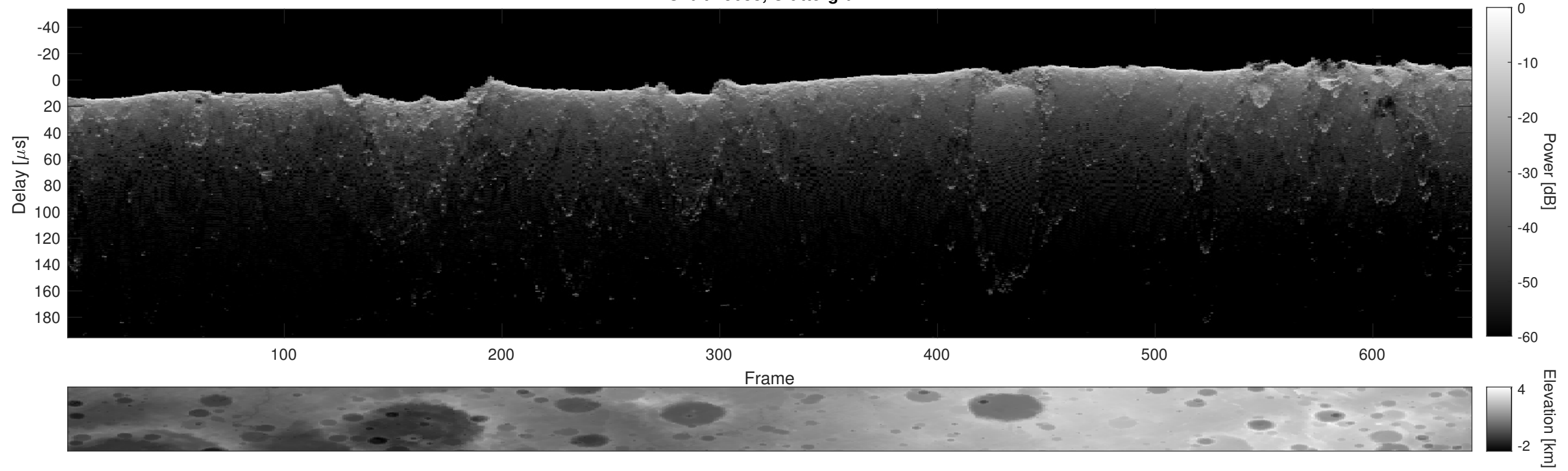
Orbit 15688, Cluttergram
