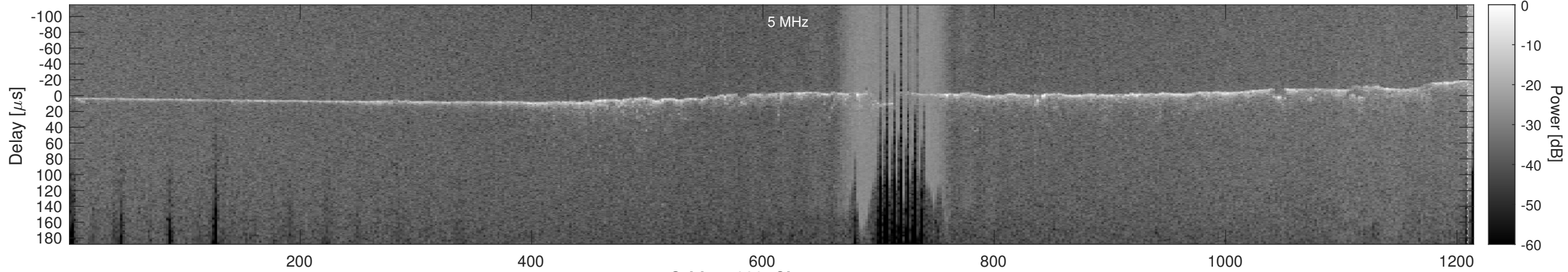
Orbit 15689, Cluttergram
