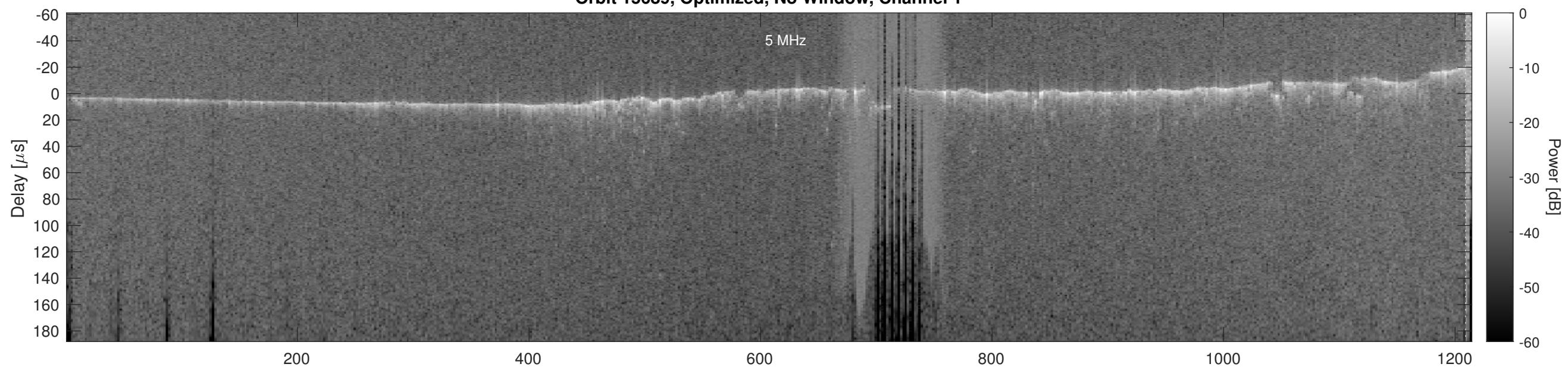
Orbit 15689, Optimized, No Window, Channel 2
