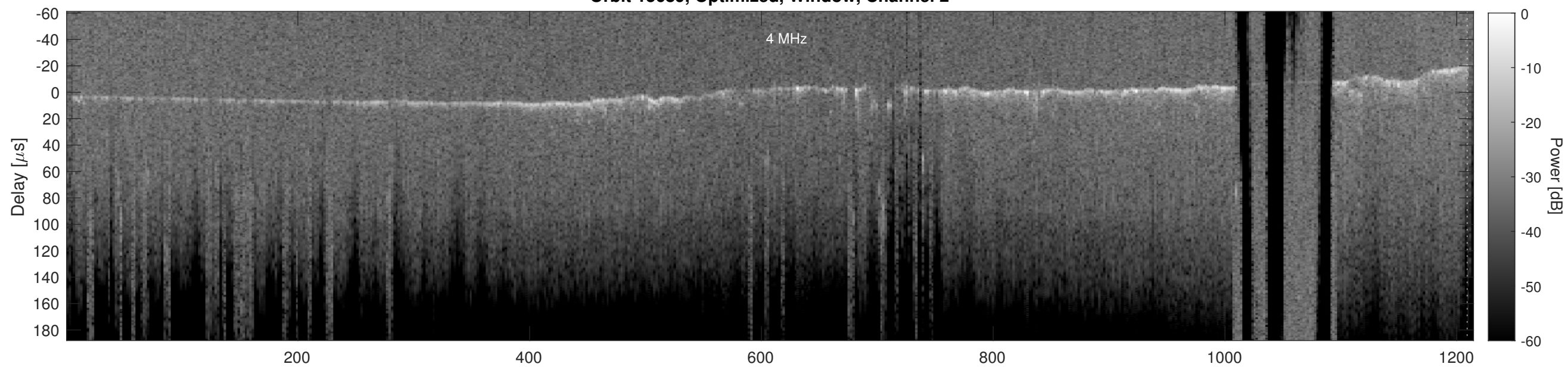
Orbit 15689, Cluttergram
