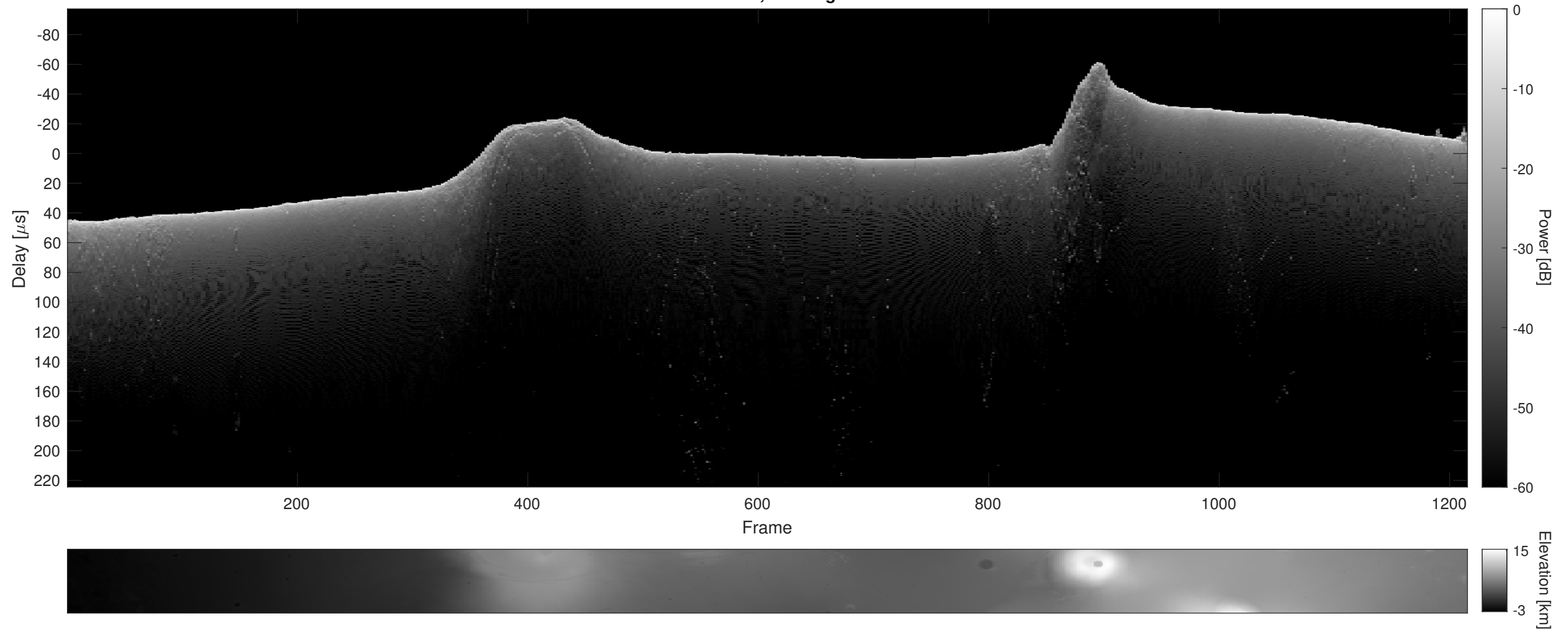
Orbit 15690, Cluttergram
