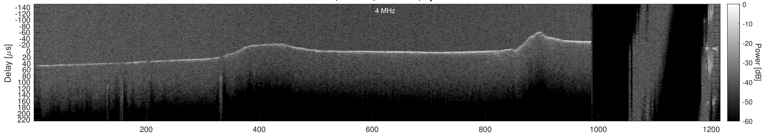
Orbit 15690, Cluttergram
