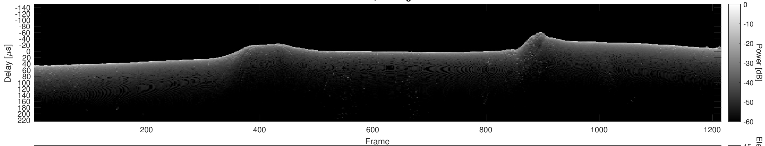
Orbit 15690, Cluttergram
