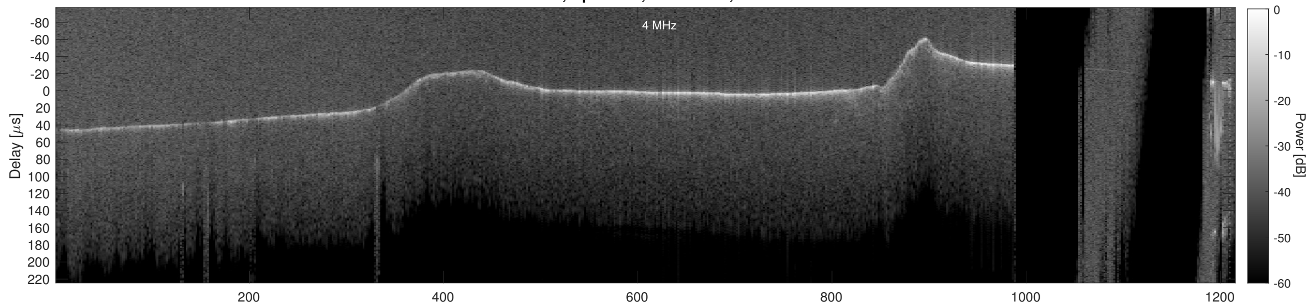
Orbit 15690, Cluttergram
