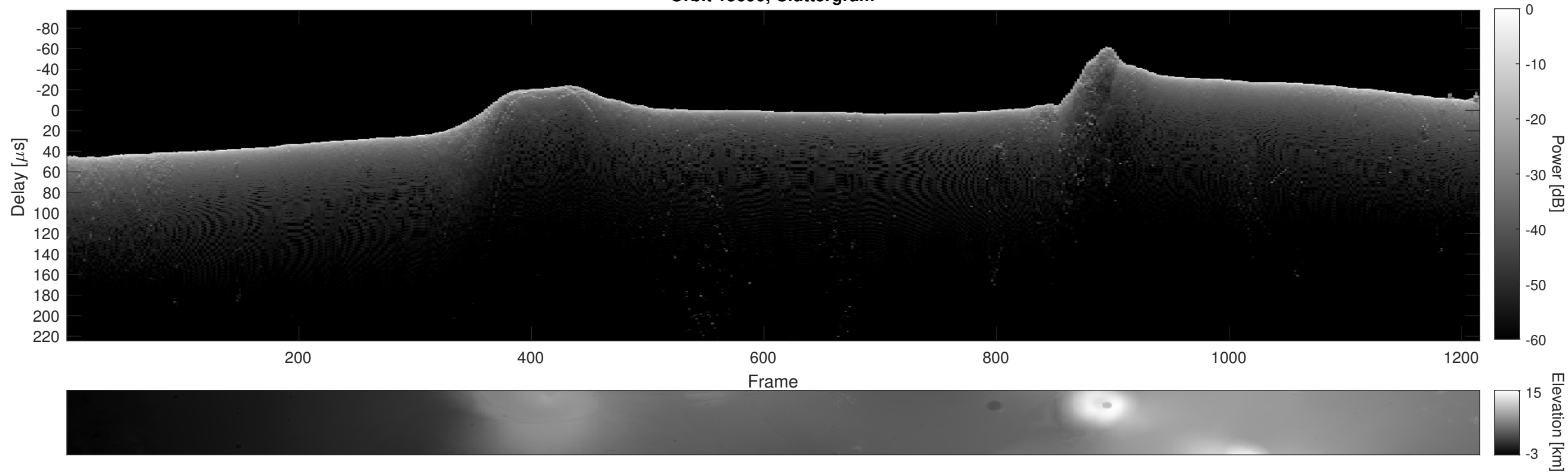
Orbit 15690, Cluttergram
