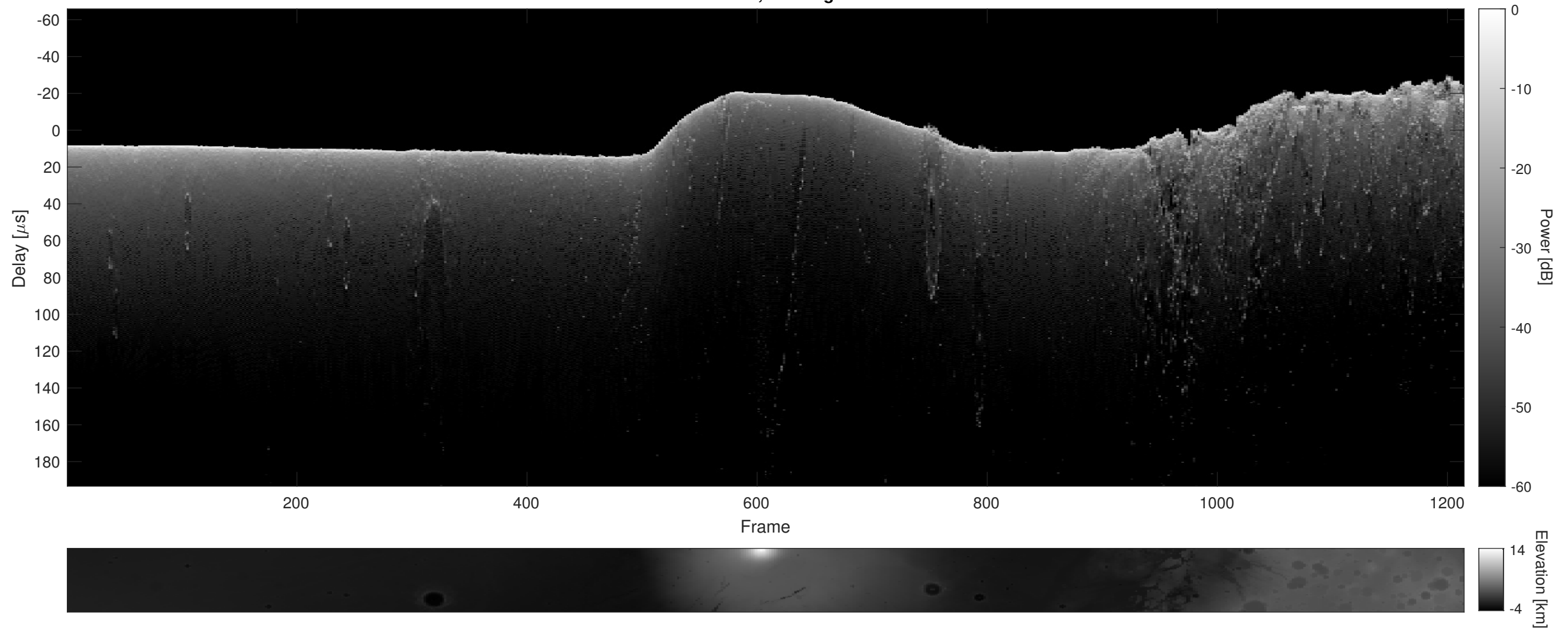
Orbit 15691, Cluttergram
