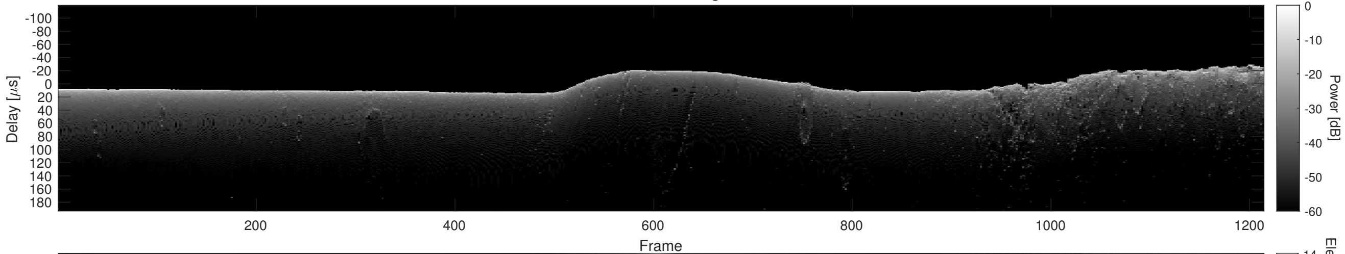
Orbit 15691, Cluttergram
