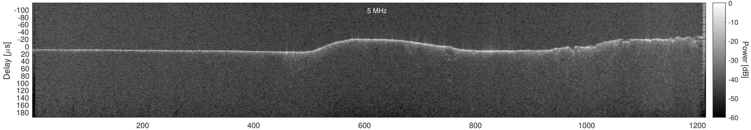
Orbit 15691, Cluttergram
