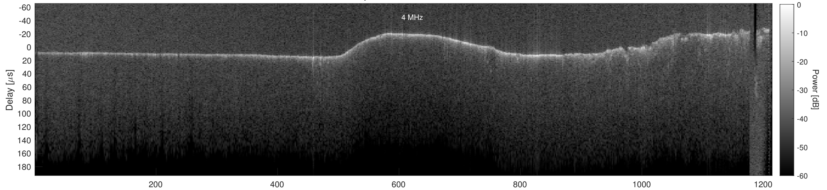
Orbit 15691, Cluttergram
