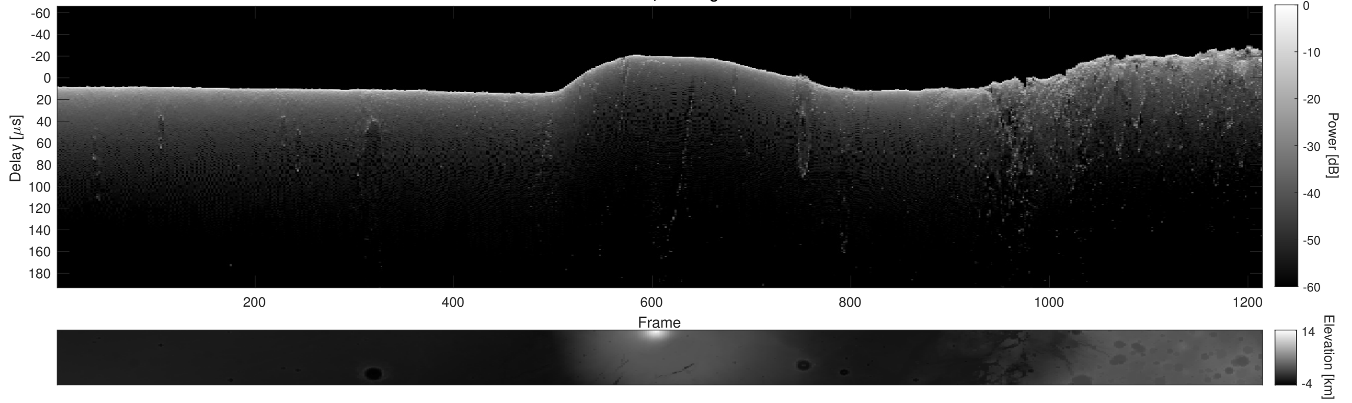
Orbit 15691, Cluttergram
