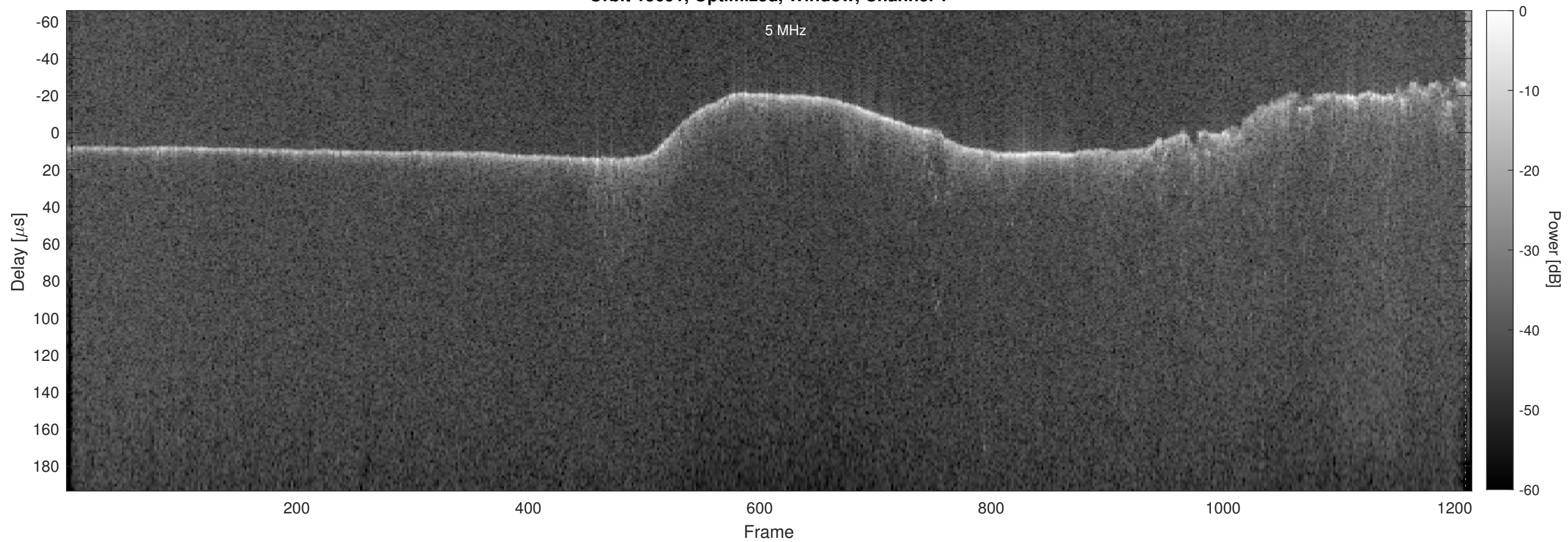
Orbit 15691, Optimized, Window, Channel 2
