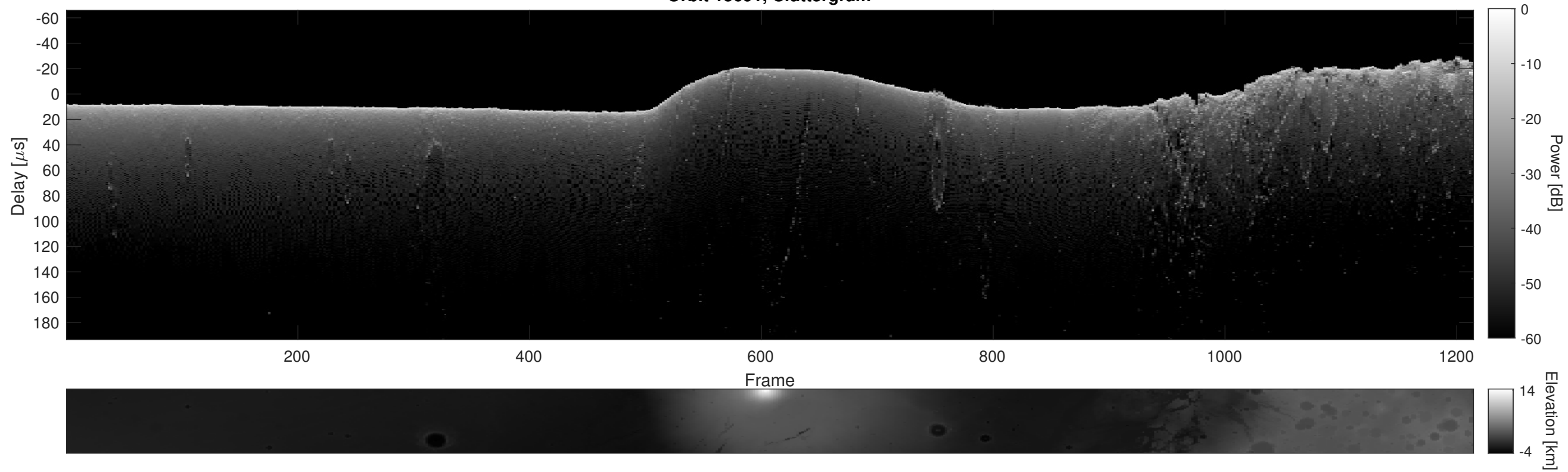
Orbit 15691, Cluttergram
