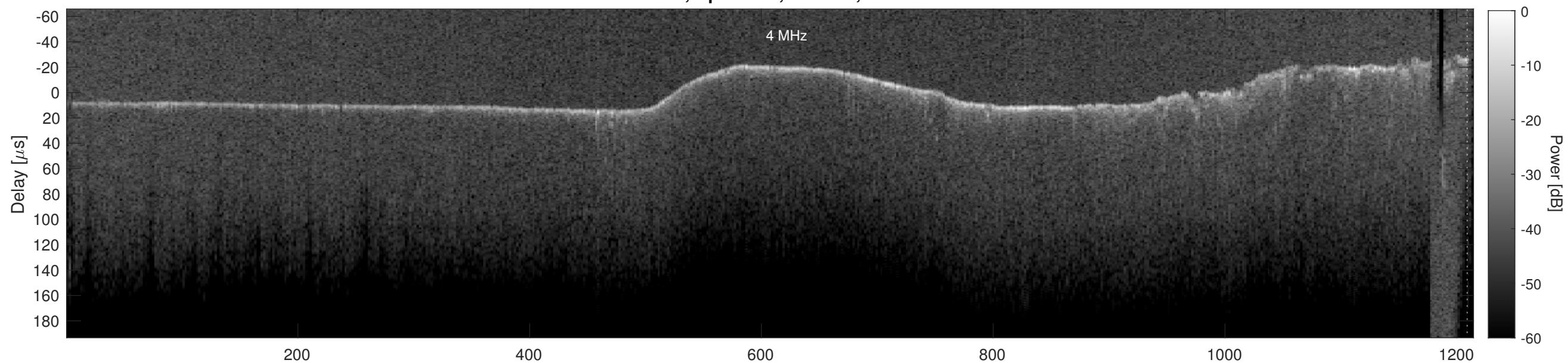
Orbit 15691, Cluttergram
