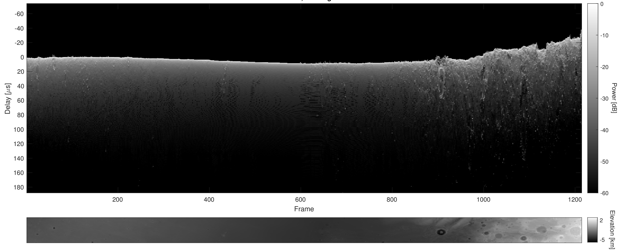
Orbit 15694, Cluttergram
