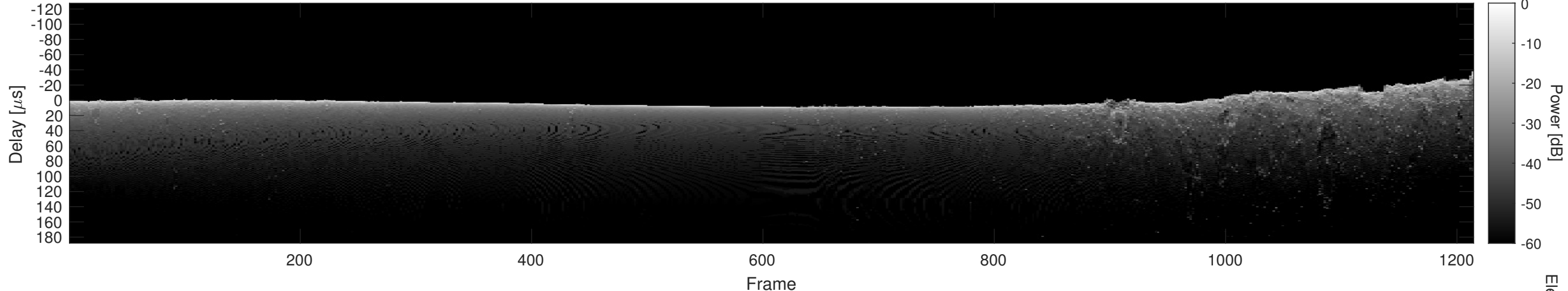
Orbit 15694, Cluttergram
