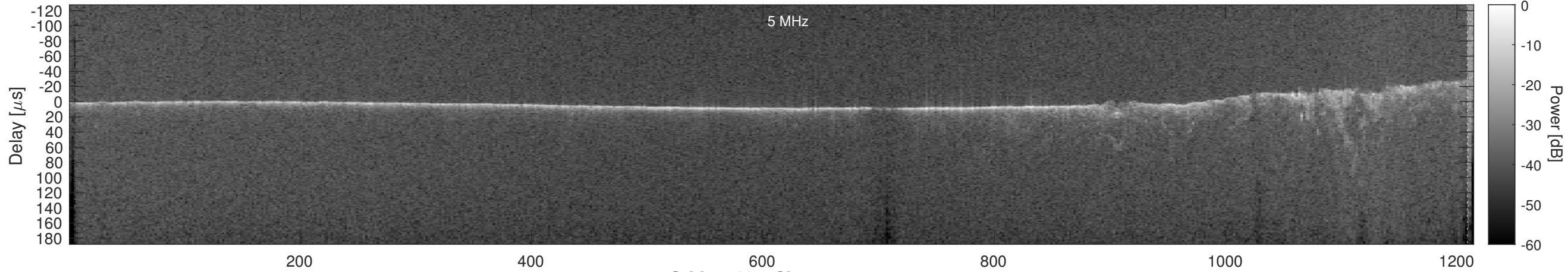
Orbit 15694, Cluttergram
