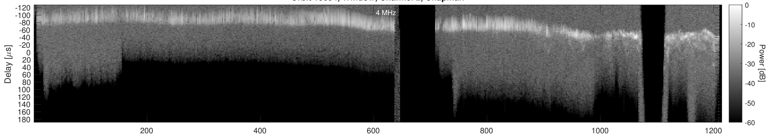
Orbit 15694, Window, Channel 2, Optimized
