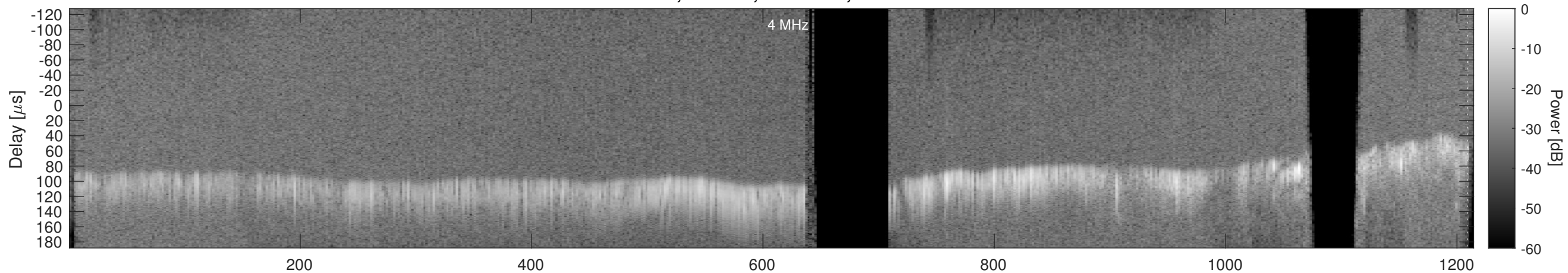
Orbit 15694, Window, Channel 2, Chapman
