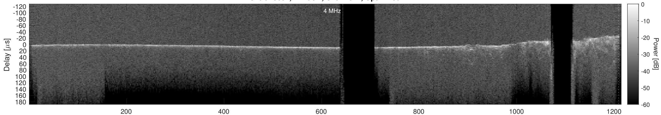
Orbit 15694, Cluttergram
