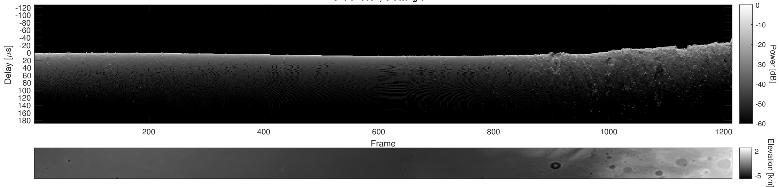
Orbit 15694, Cluttergram
