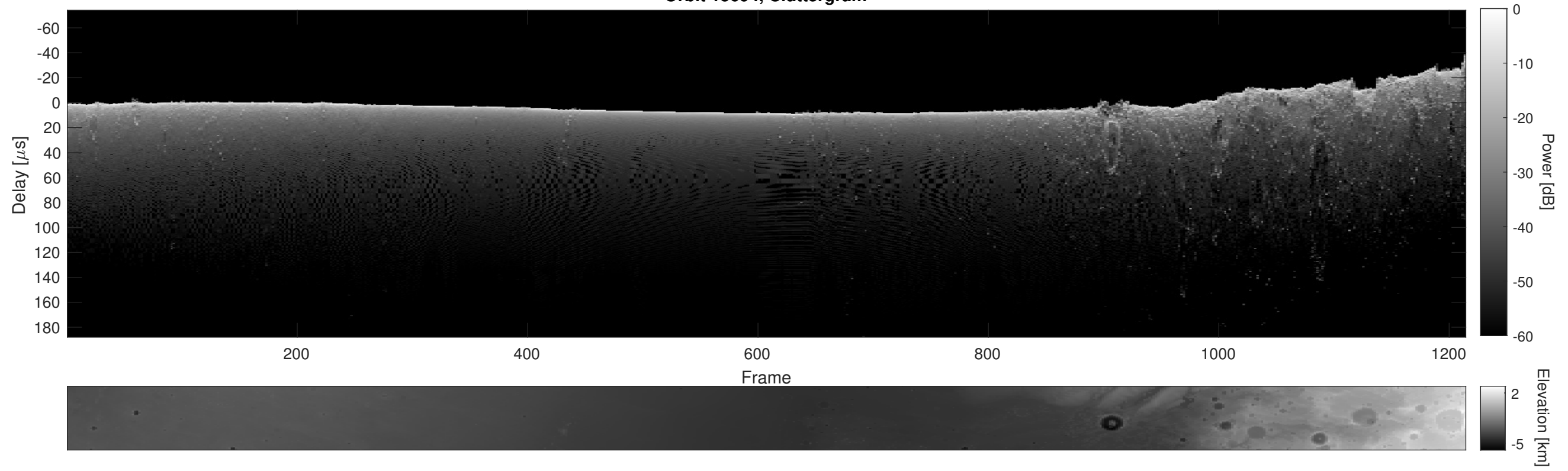
Orbit 15694, Cluttergram
