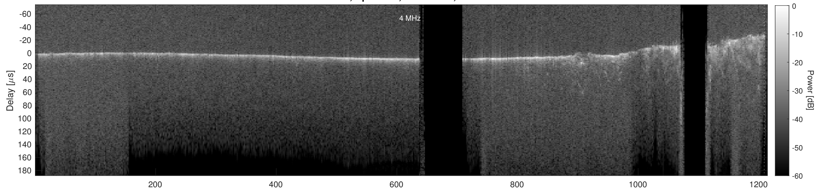
Orbit 15694, Cluttergram
