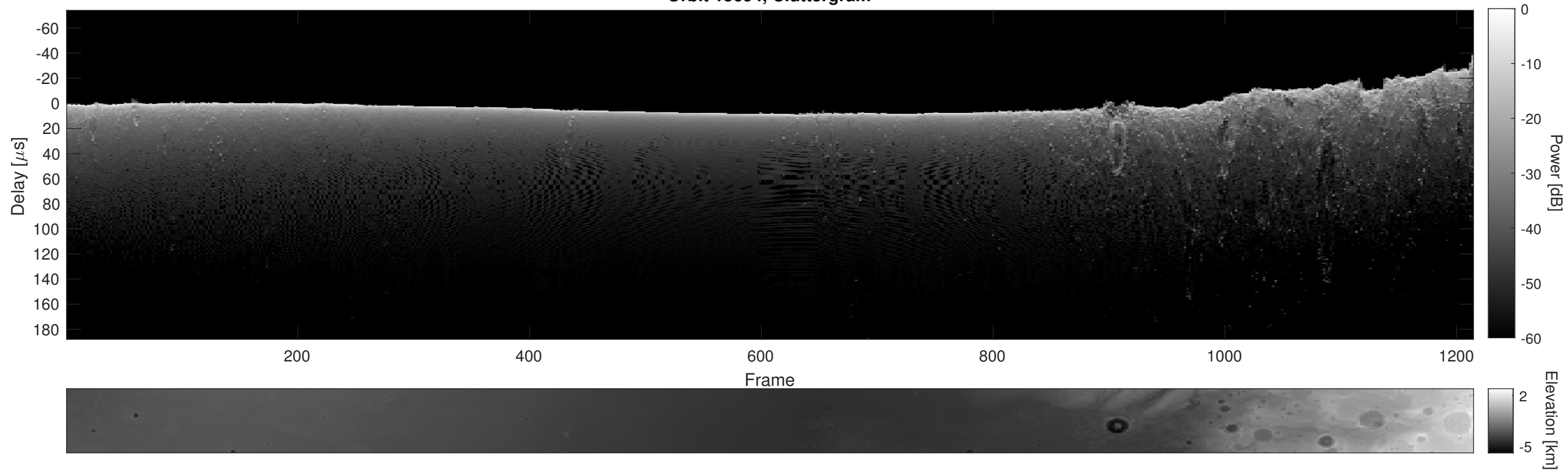
Orbit 15694, Cluttergram
