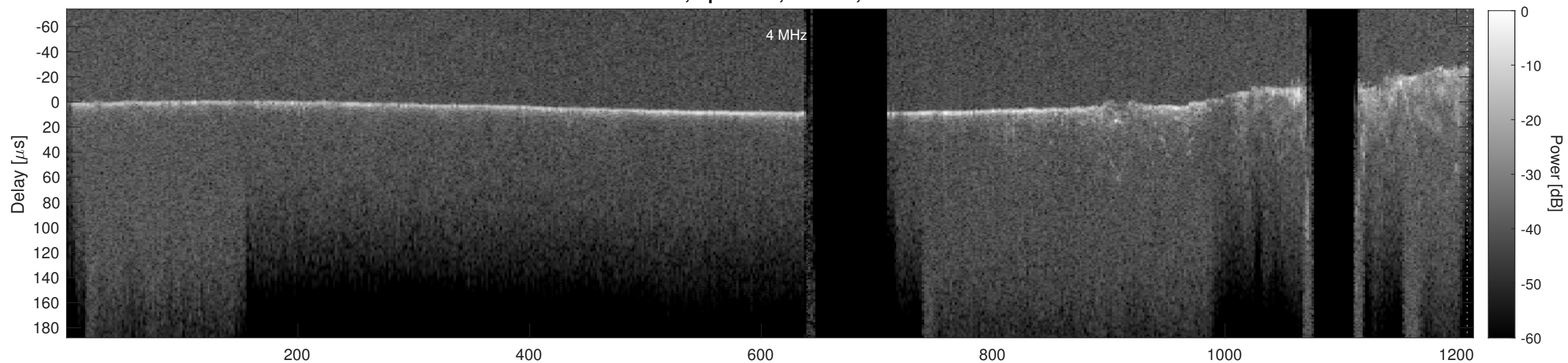
Orbit 15694, Cluttergram
