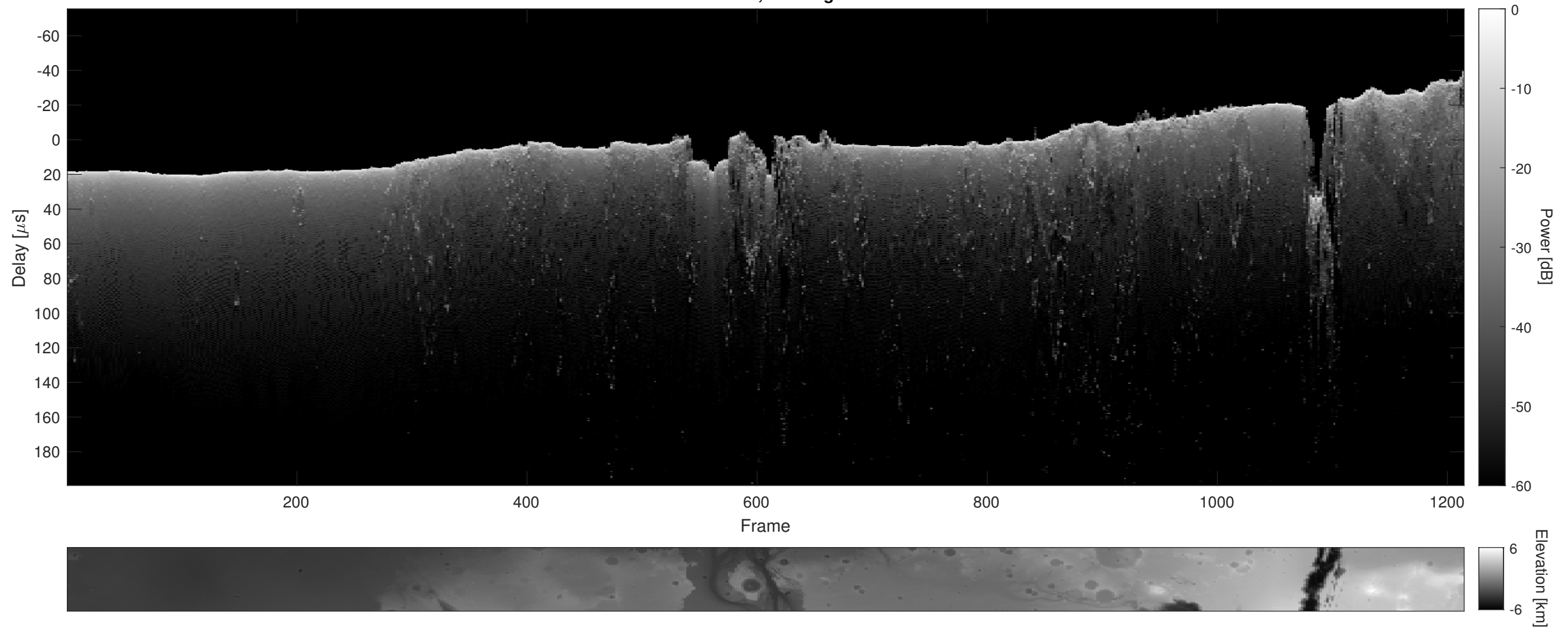
Orbit 15700, Cluttergram
