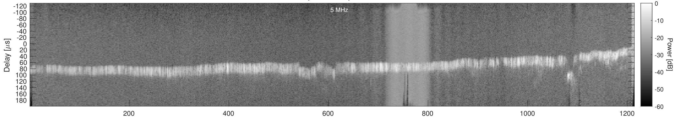
Orbit 15700, Window, Channel 1, Chapman
