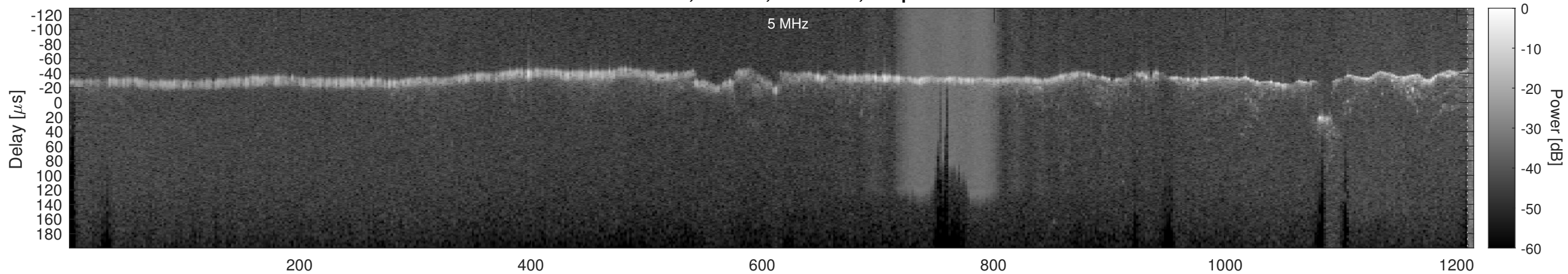
Orbit 15700, Window, Channel 1, Optimized
