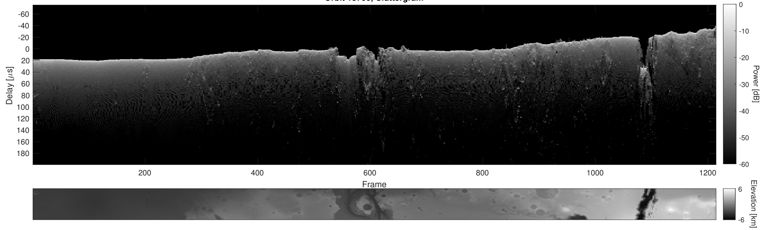
Orbit 15700, Cluttergram
