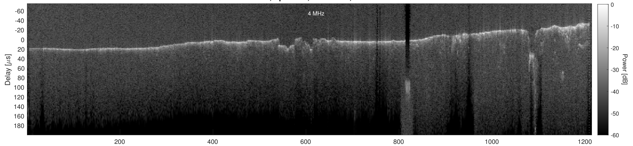
Orbit 15700, Cluttergram
