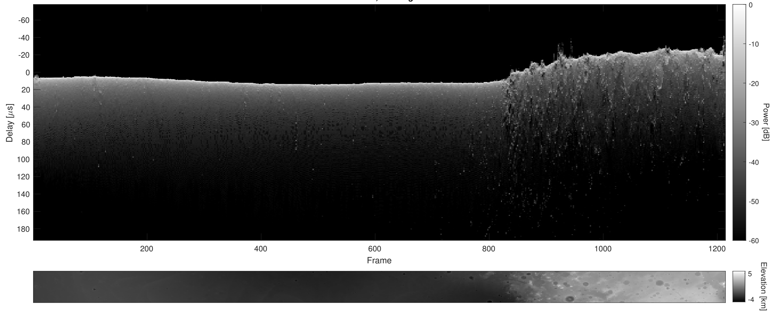
Orbit 15702, Cluttergram
