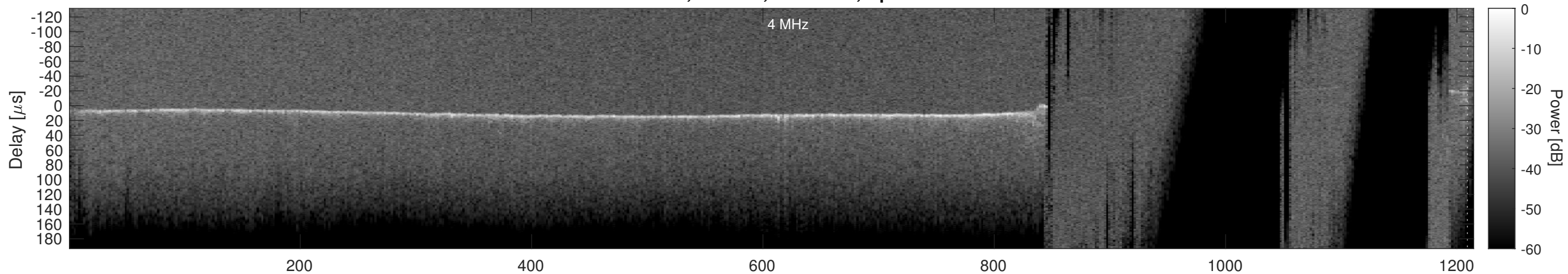
Orbit 15702, Cluttergram
