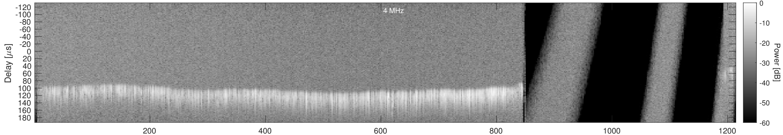
Orbit 15702, Window, Channel 2, Chapman
