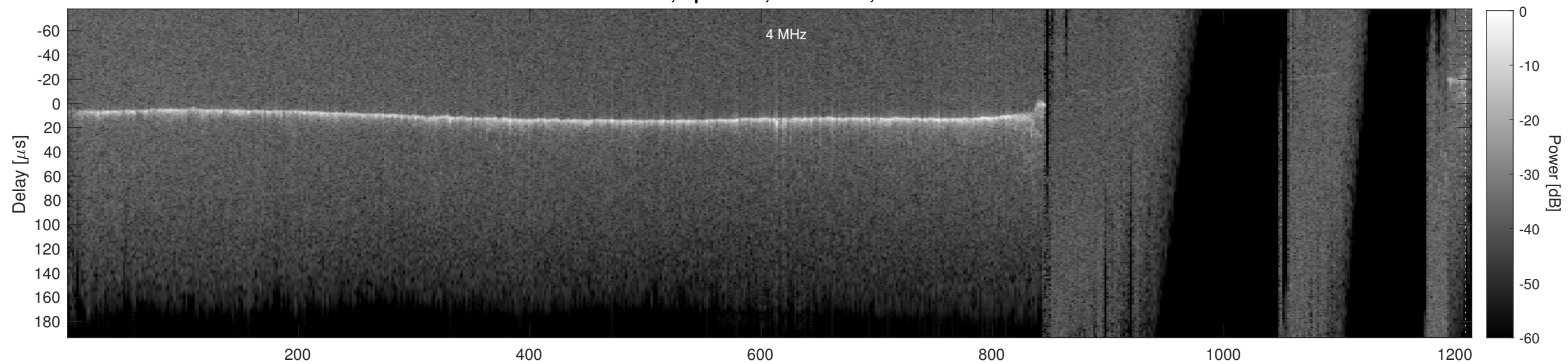
Orbit 15702, Cluttergram
