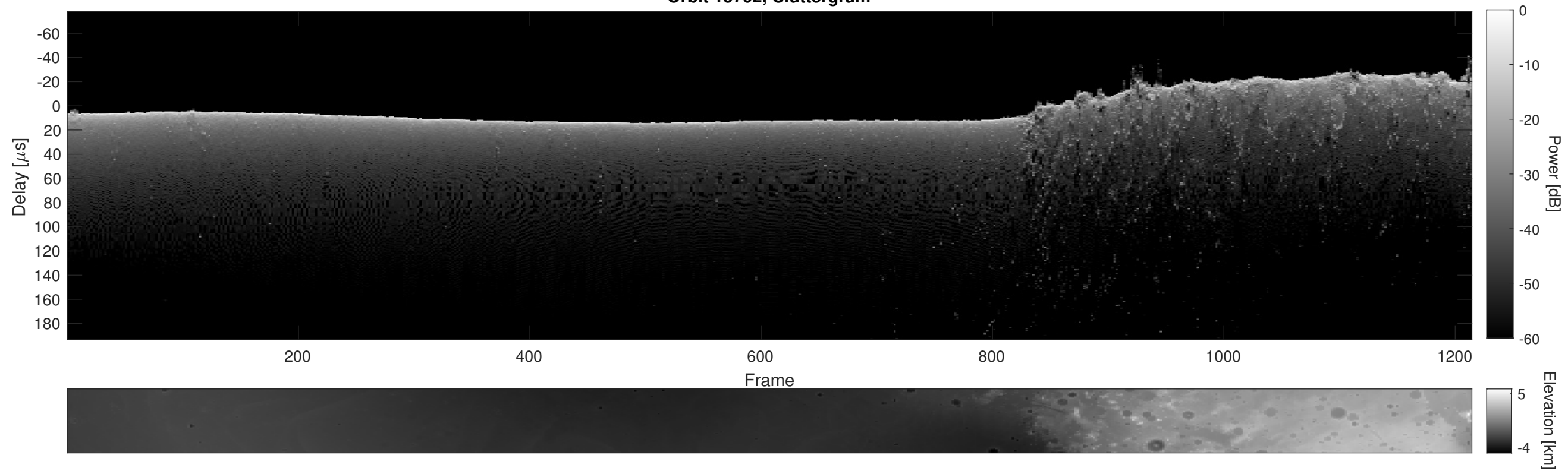
Orbit 15702, Cluttergram
