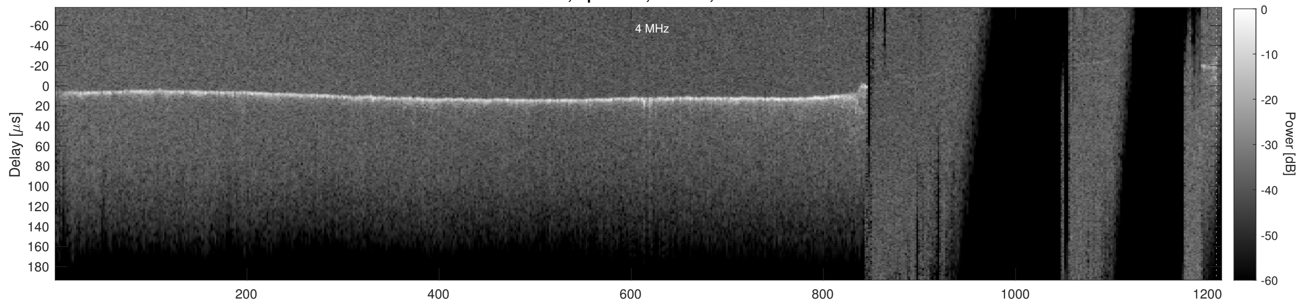
Orbit 15702, Cluttergram
