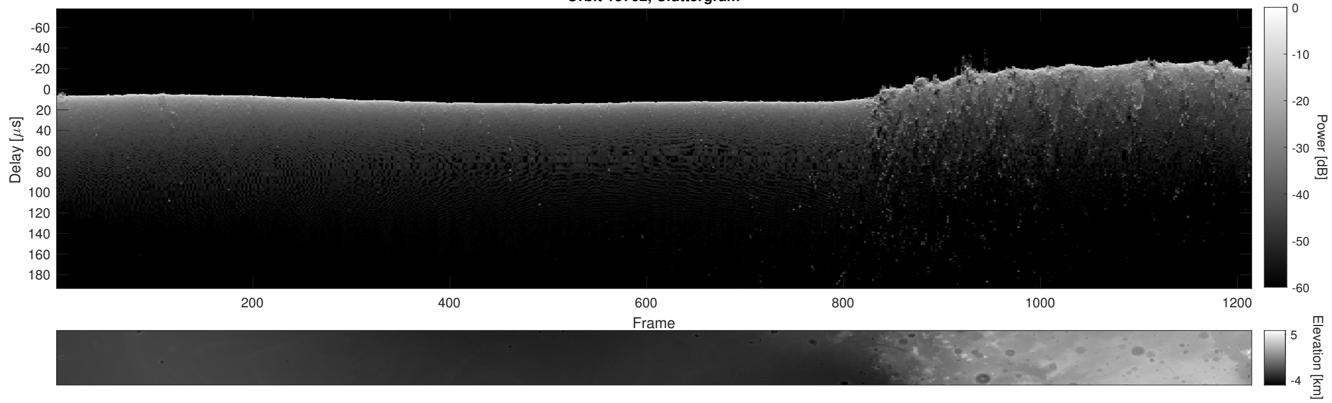
Orbit 15702, Cluttergram
