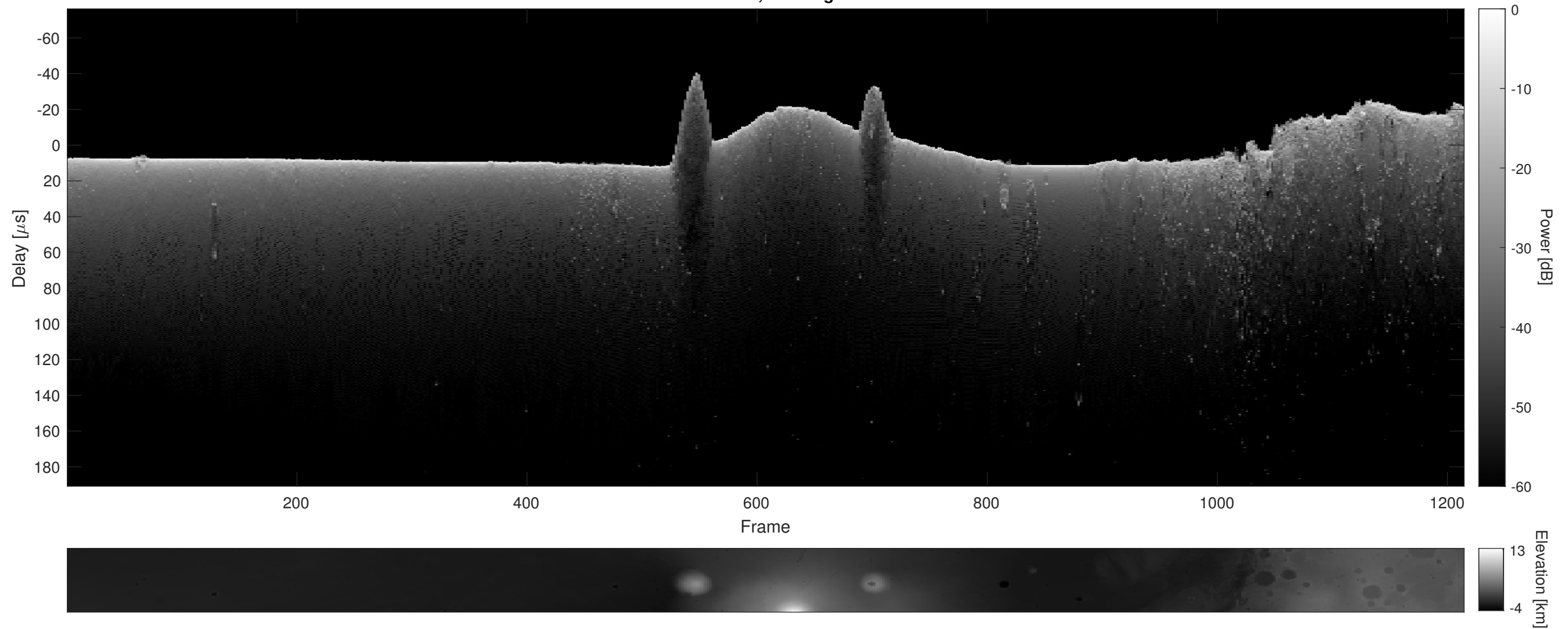
Orbit 15705, Cluttergram
