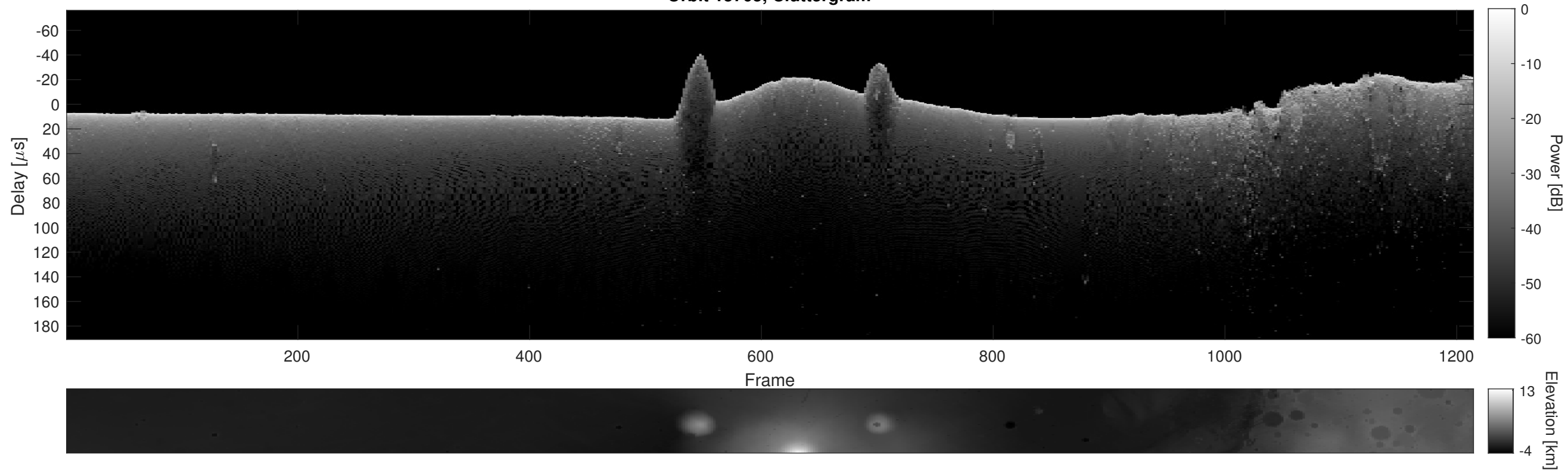
Orbit 15705, Cluttergram
