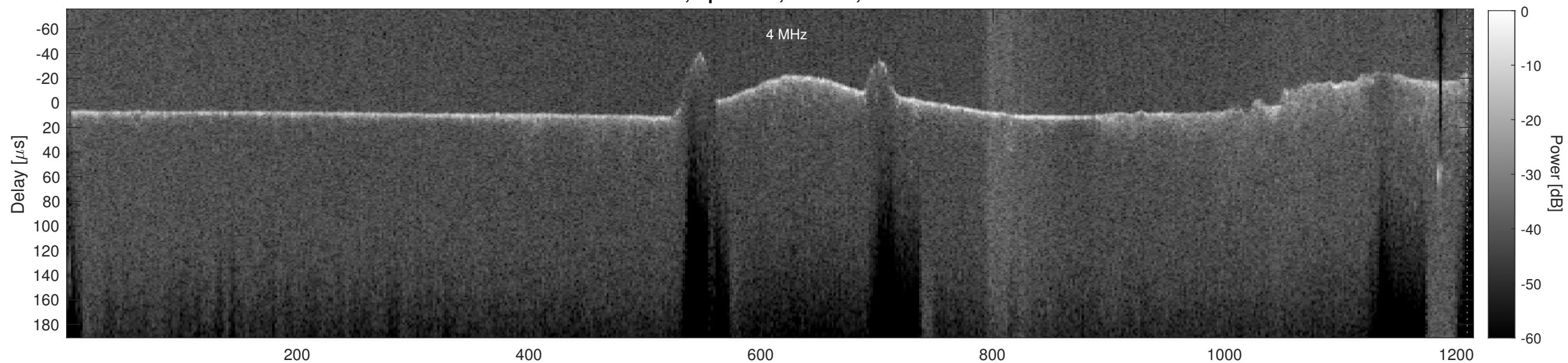
Orbit 15705, Cluttergram
