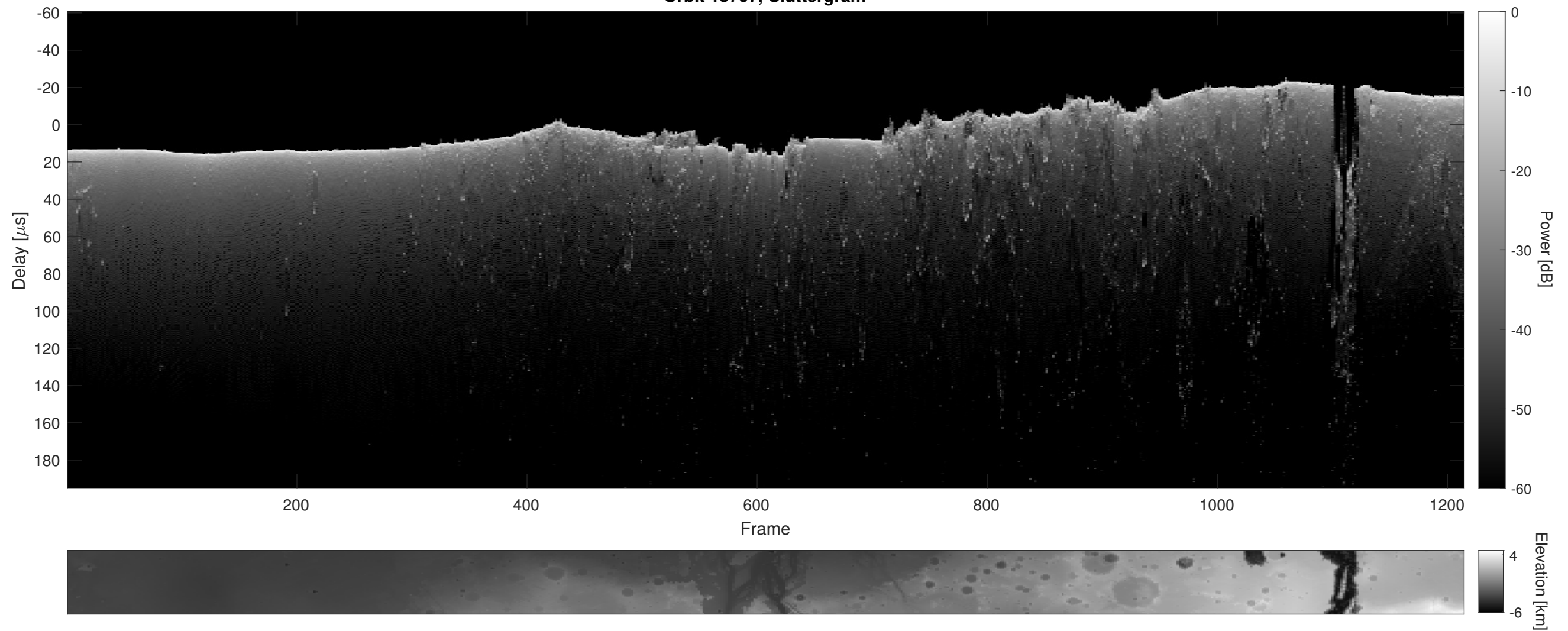
Orbit 15707, Cluttergram
