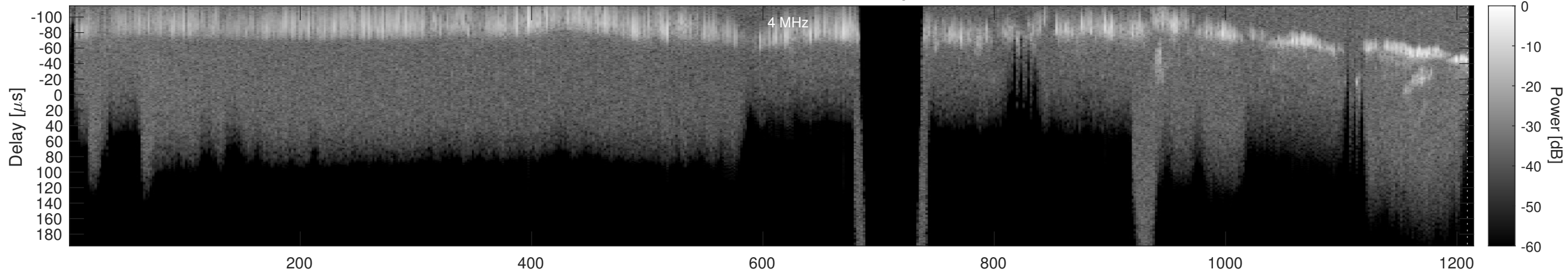
Orbit 15707, Window, Channel 2, Optimized
