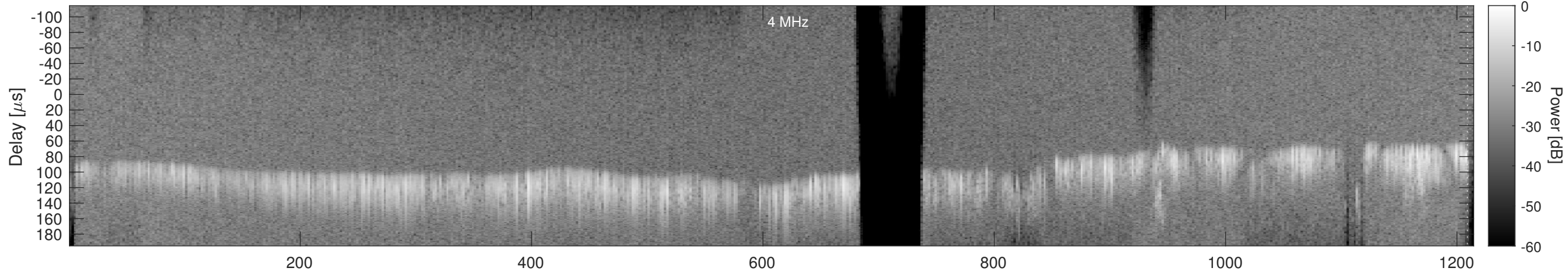
Orbit 15707, Window, Channel 2, Chapman
