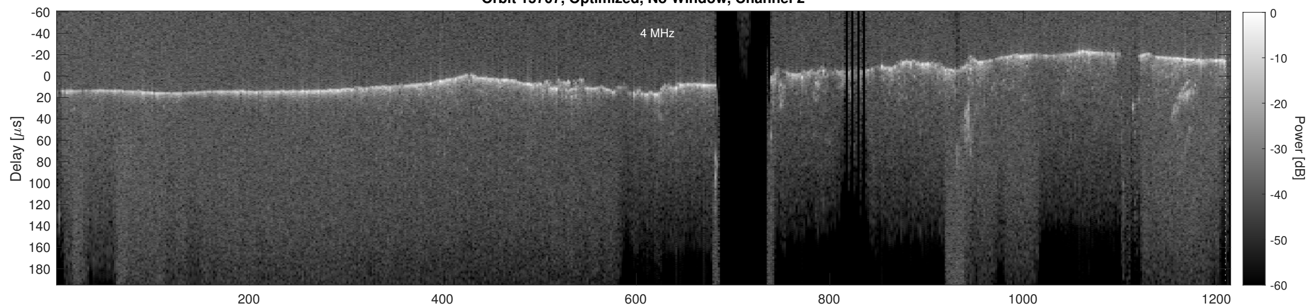
Orbit 15707, Cluttergram
