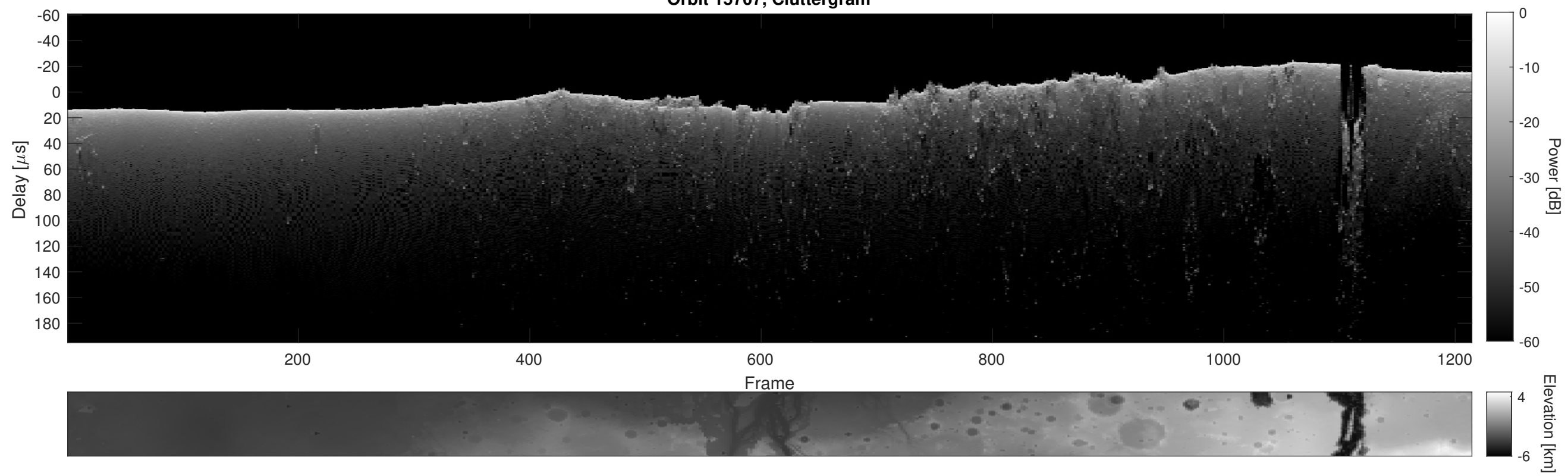
Orbit 15707, Cluttergram
