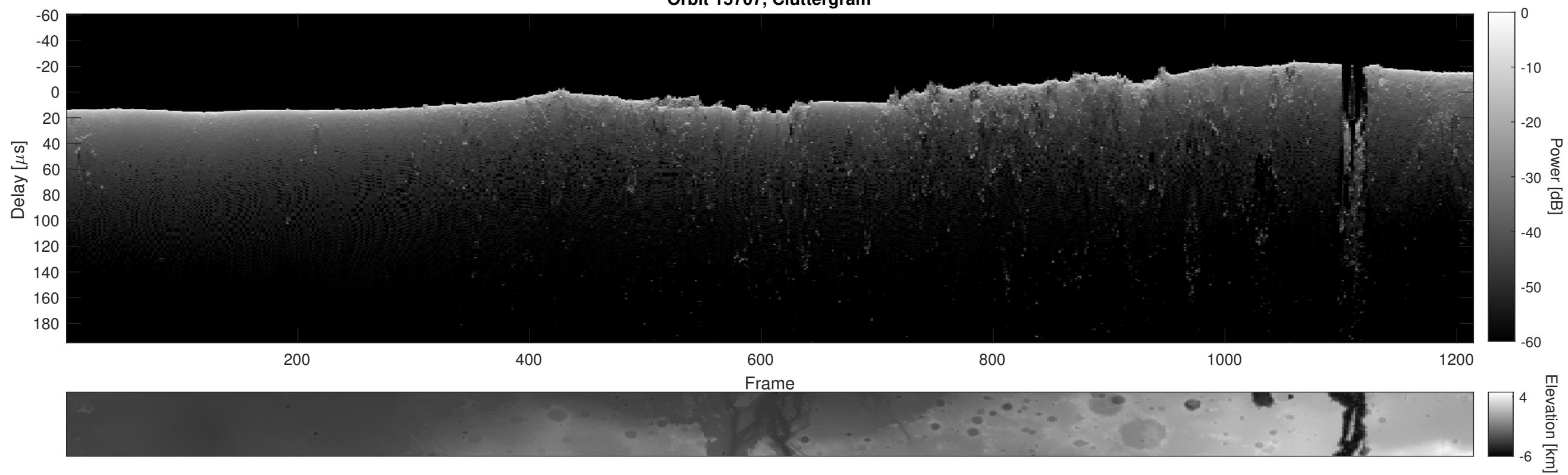
Orbit 15707, Cluttergram
