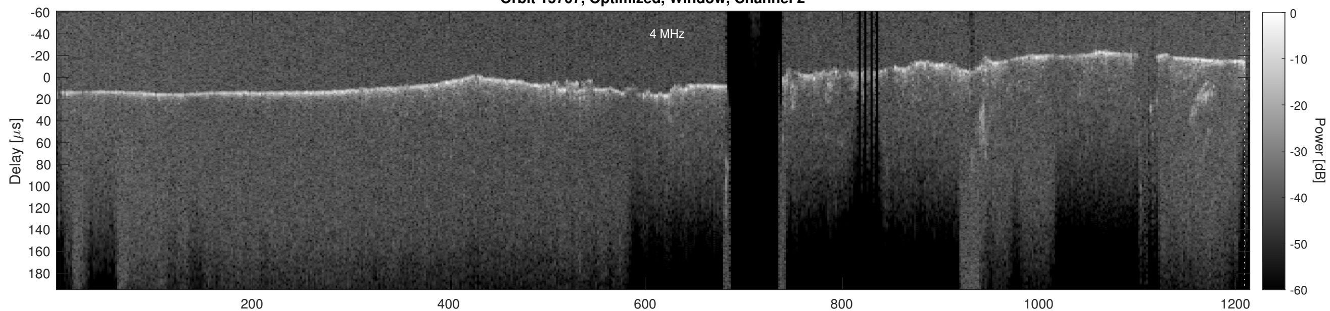
Orbit 15707, Cluttergram
